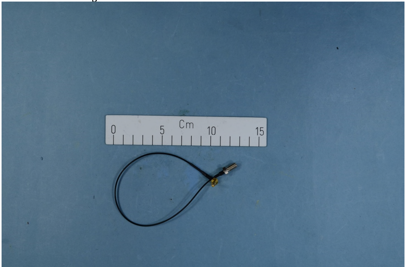
FL connector to SMA for conducted radio measurements
