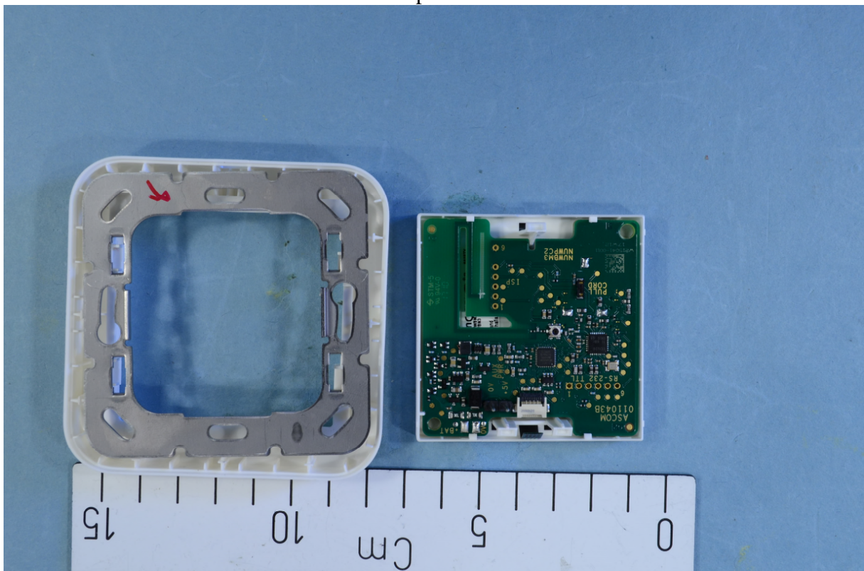
Bottom view of the board with casing
