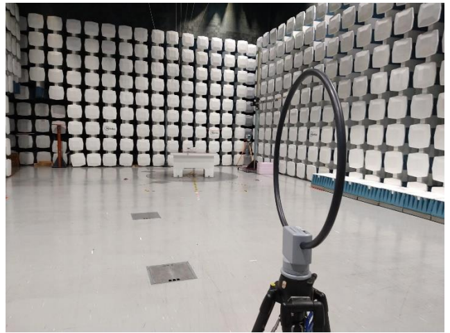
Radiated emissions < 30MHz, Longitudinal
