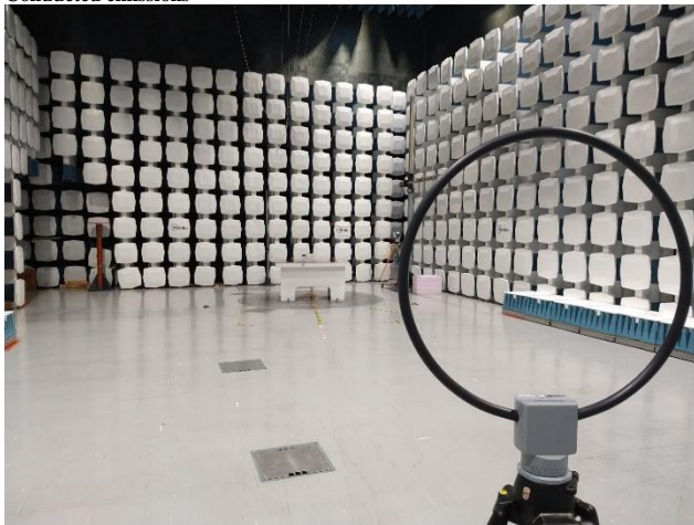
Radiated emissions < 30MHz, Transverse
