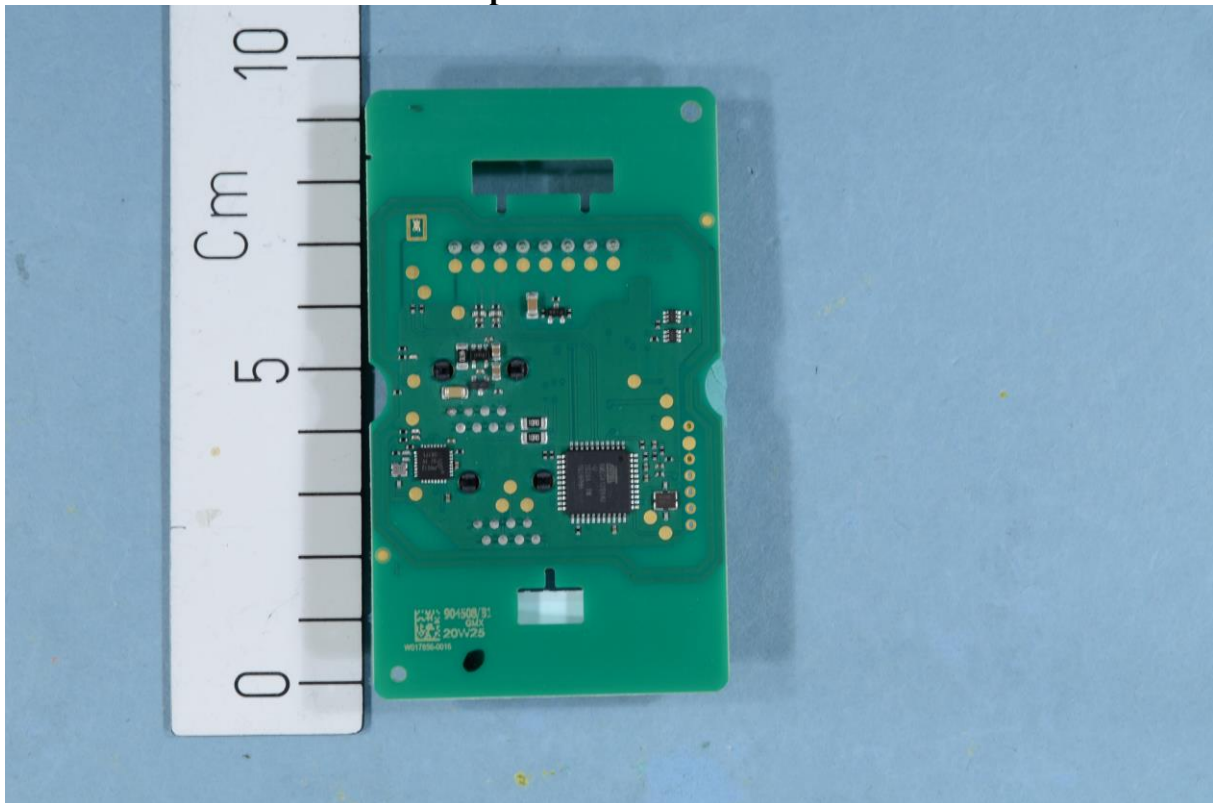
Rear view – main board
