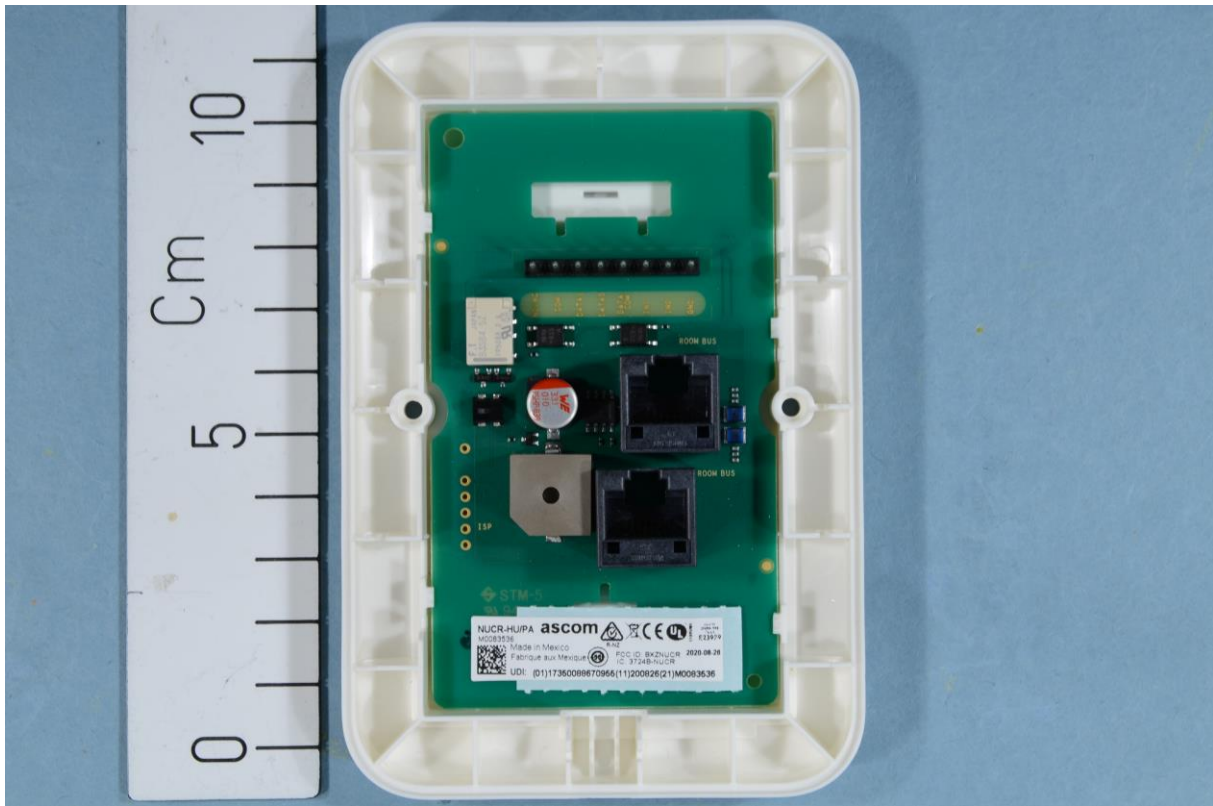
Top view – main board
