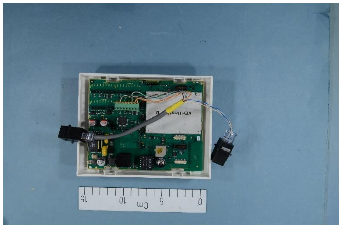
Auxiliary device NIRC4 as power supply to the bus
