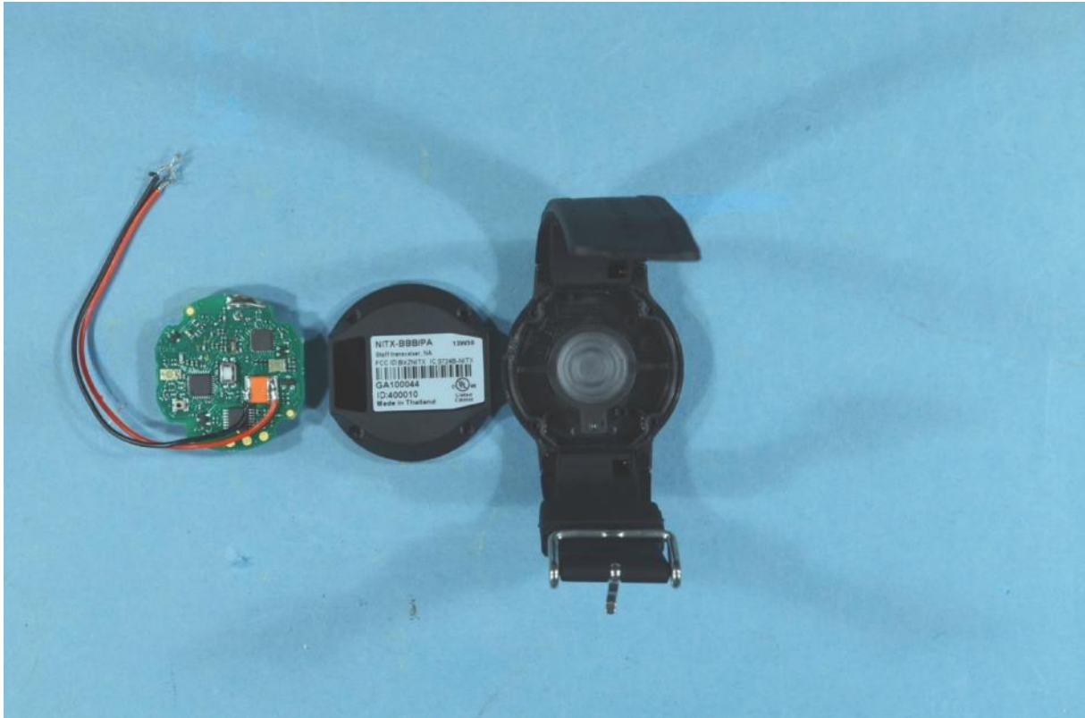
NITX with cover
