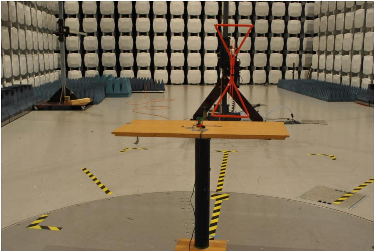
Radiated Emissions 30 - 1000 MHz, 3 meter – In RX mode
