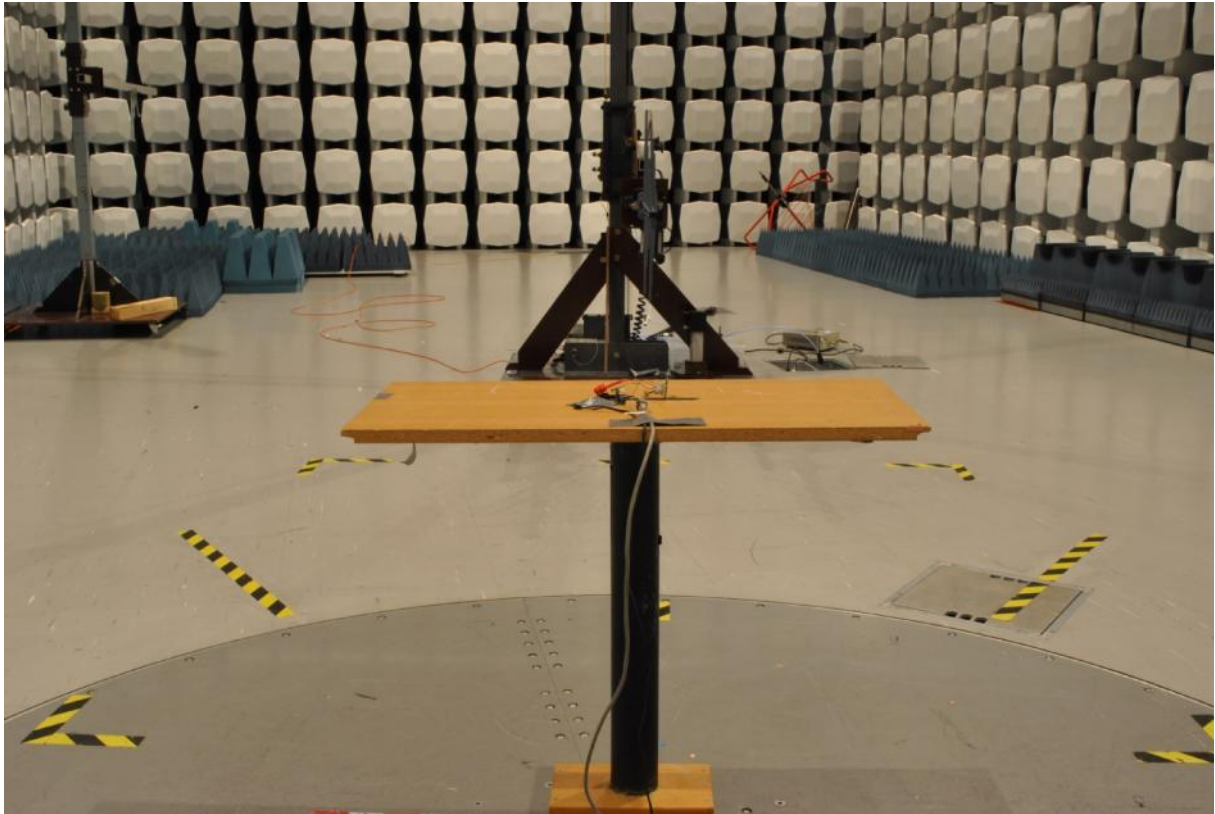
Radiated Emissions 30 - 1000 MHz, 3 meter – In TX mode
