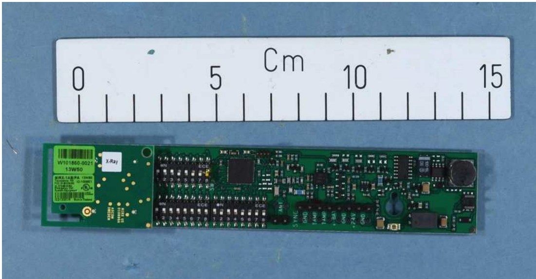
NIRX mounted on test-jig
