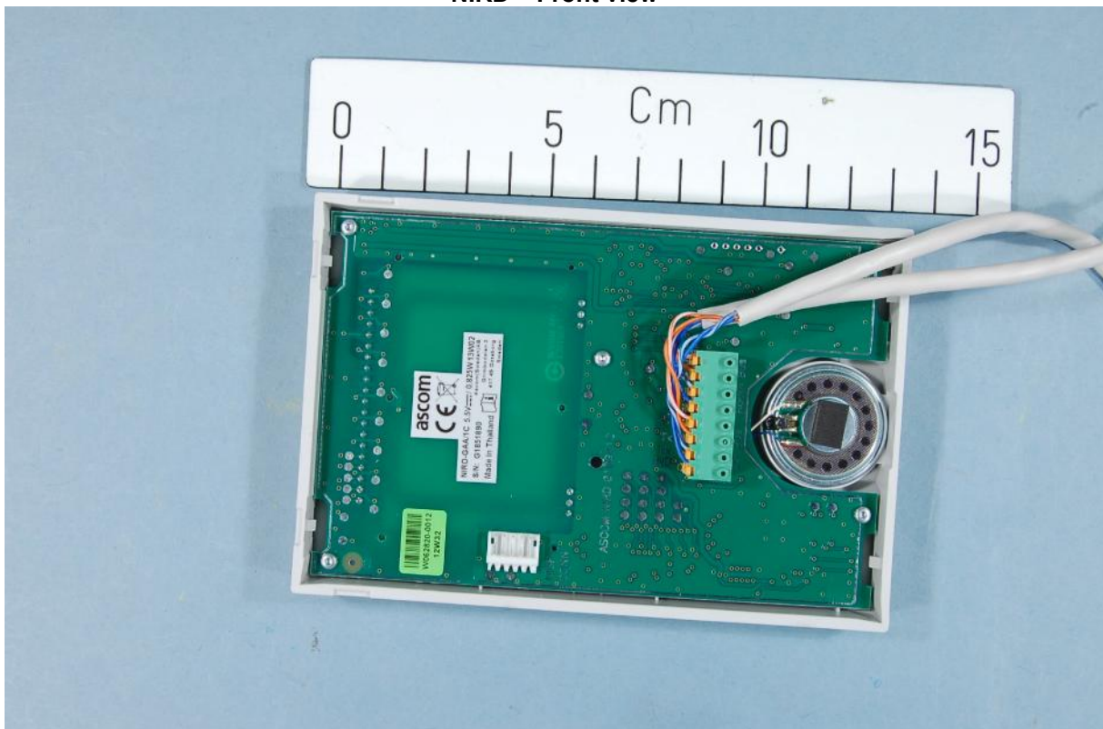
NIRD – Rear View
