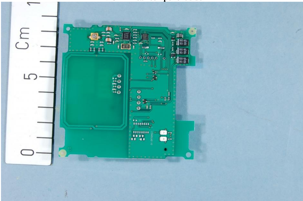
NICR – Loop antenna side
