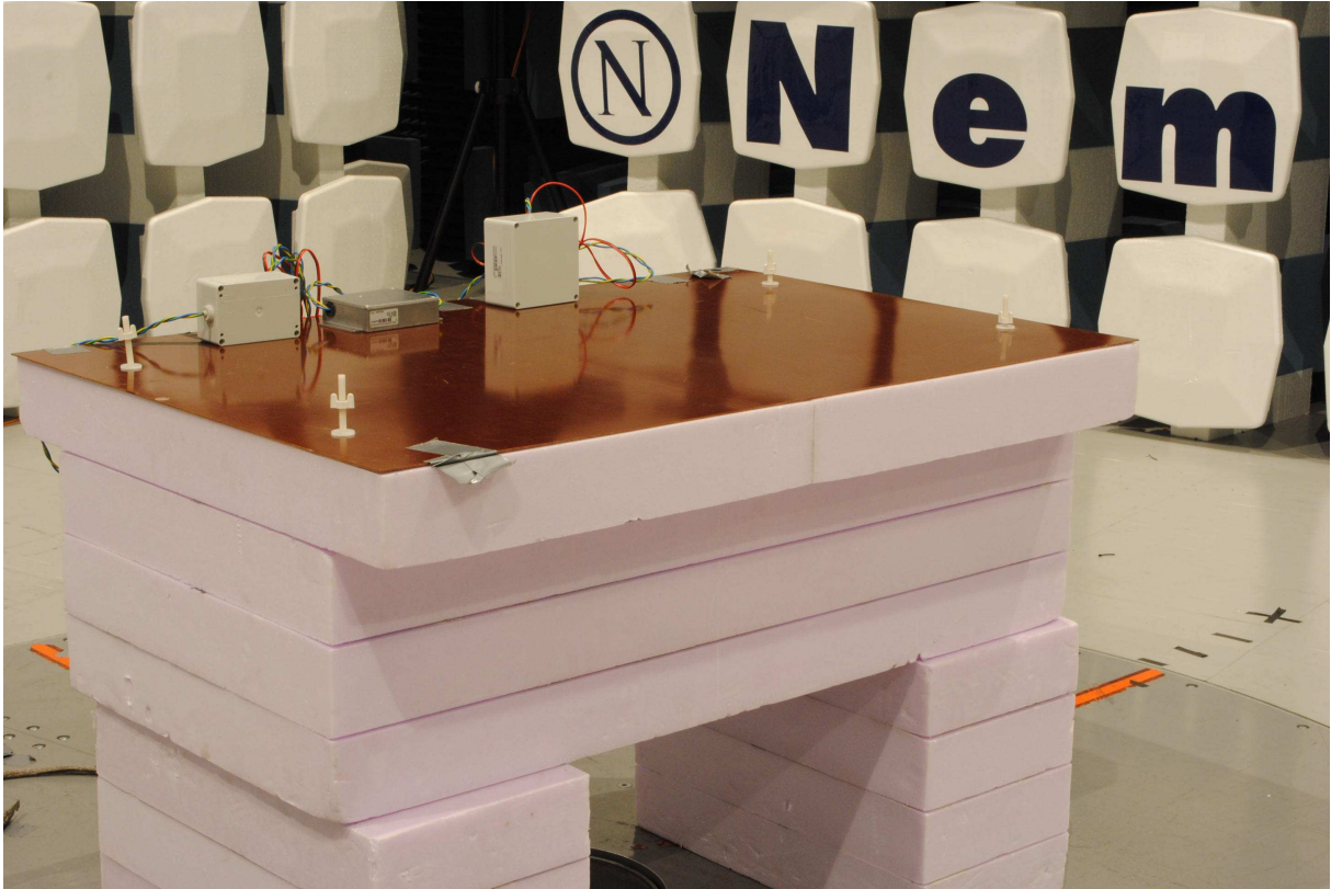
Radiated emission 30 - 1000MHz Test Set-up
