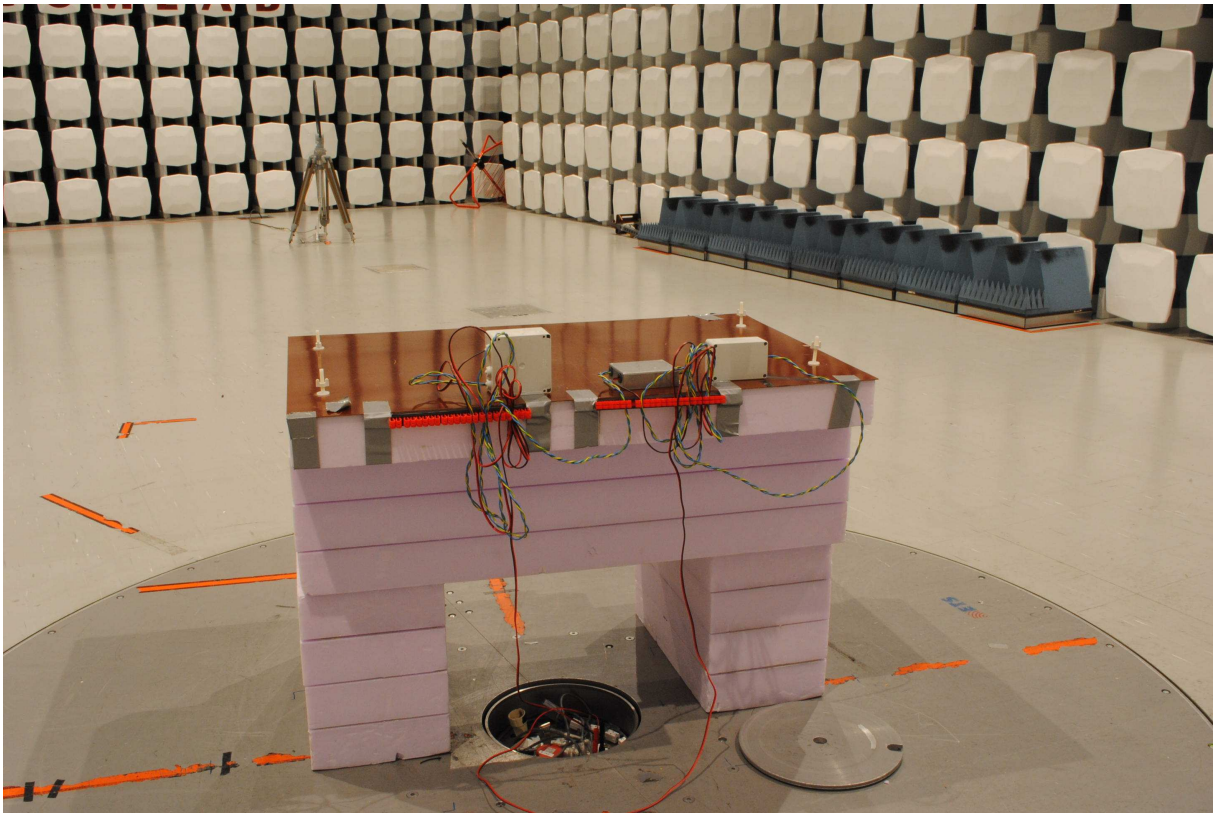
Radiated emission 9kHz - 30MHz Test Set-up
