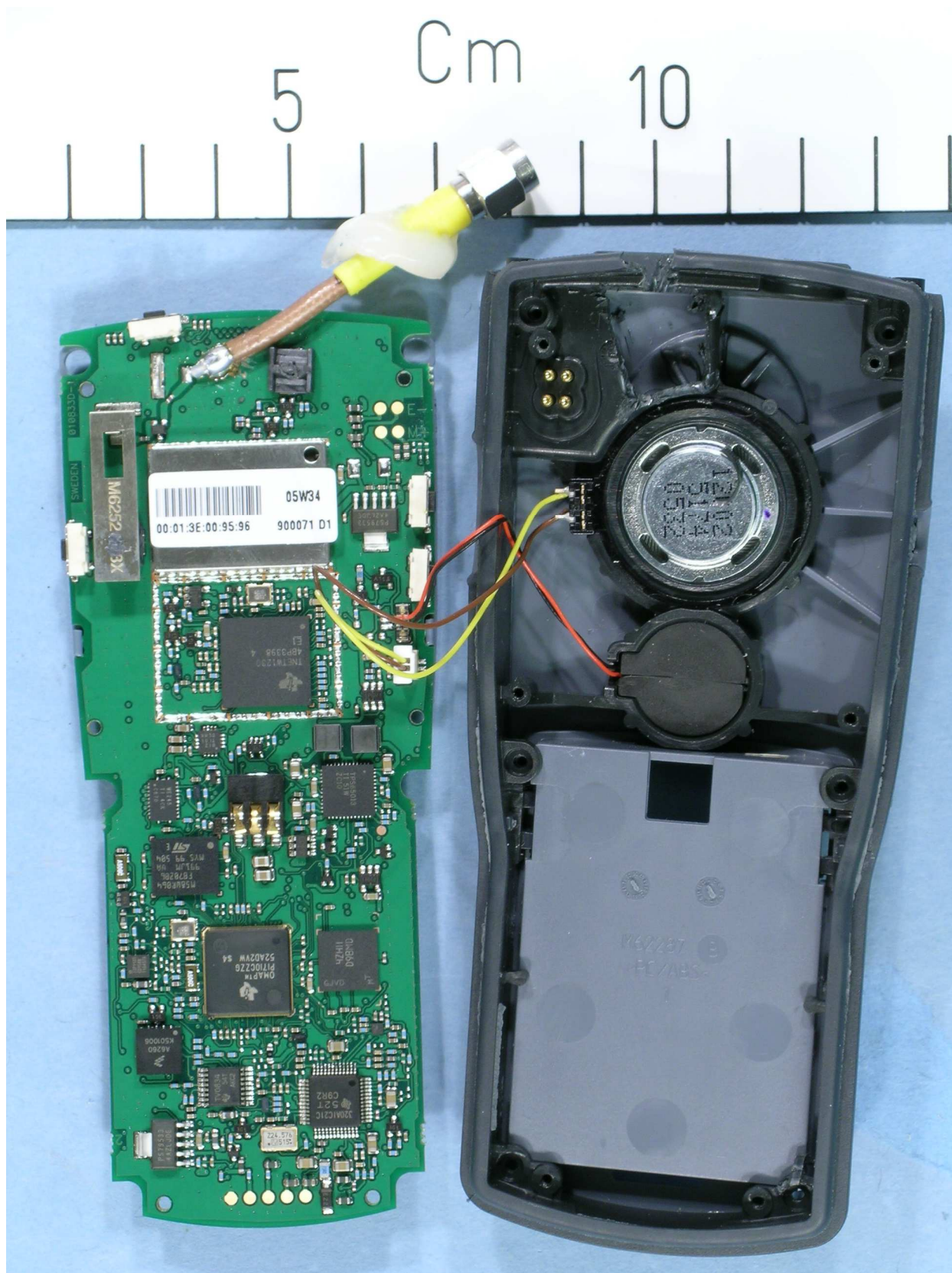
Ascom KATY WLAN Handset, Conducted sample
