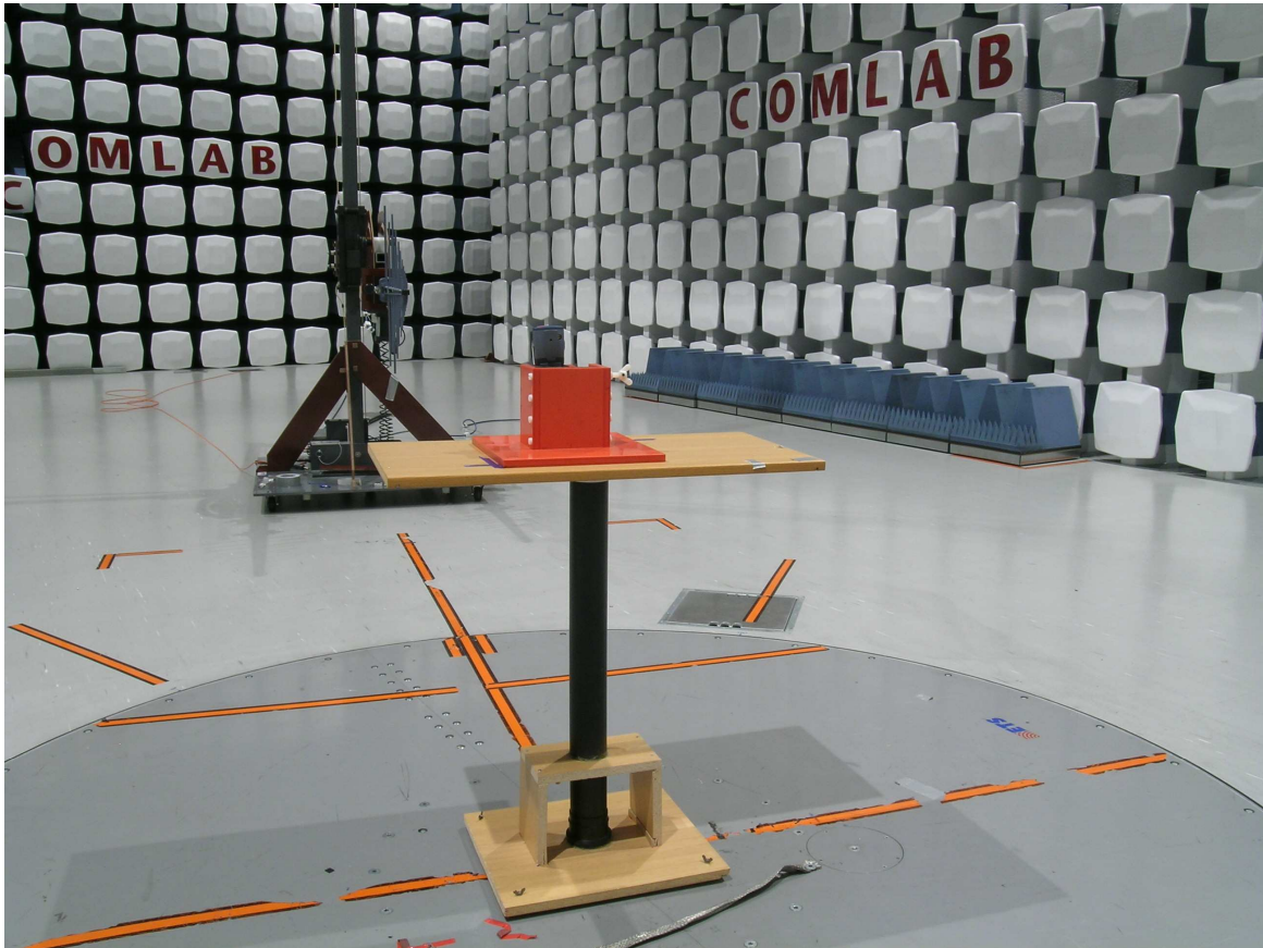
Test setup 200 – 1000 MHz Radiated
