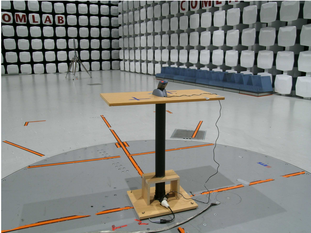
Test Setup radiated < 30 MHz
