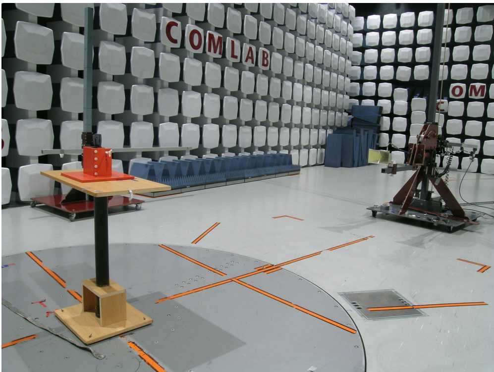
Test setup Radiated 1 – 8.5 GHz
