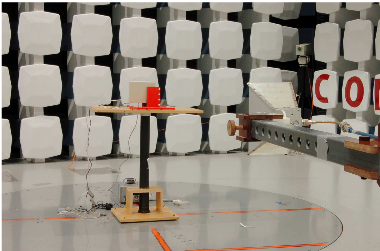
ASCOM IPBS1 - Radiated emissions 1 GHz – 8.5 GHz
