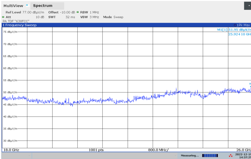
Pre-scan 18 - 26 GHz, 2441 MHz, π/4-DQPSK, @10cm
