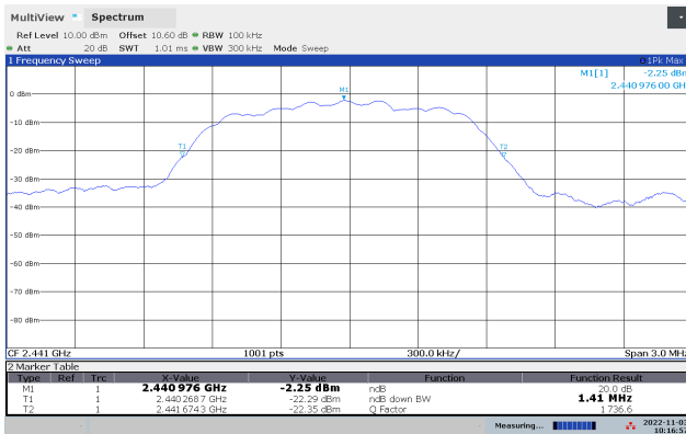
20dB Bandwidth 2441 MHz, 8-DPSK
