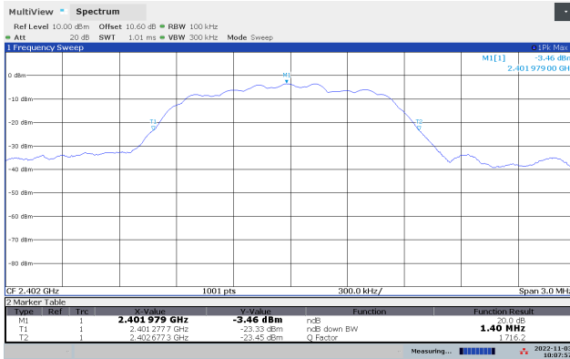
20dB Bandwidth 2402 MHz, 8-DPSK
