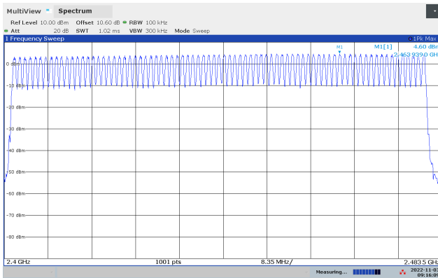
RF Channels in Use, GFSK
