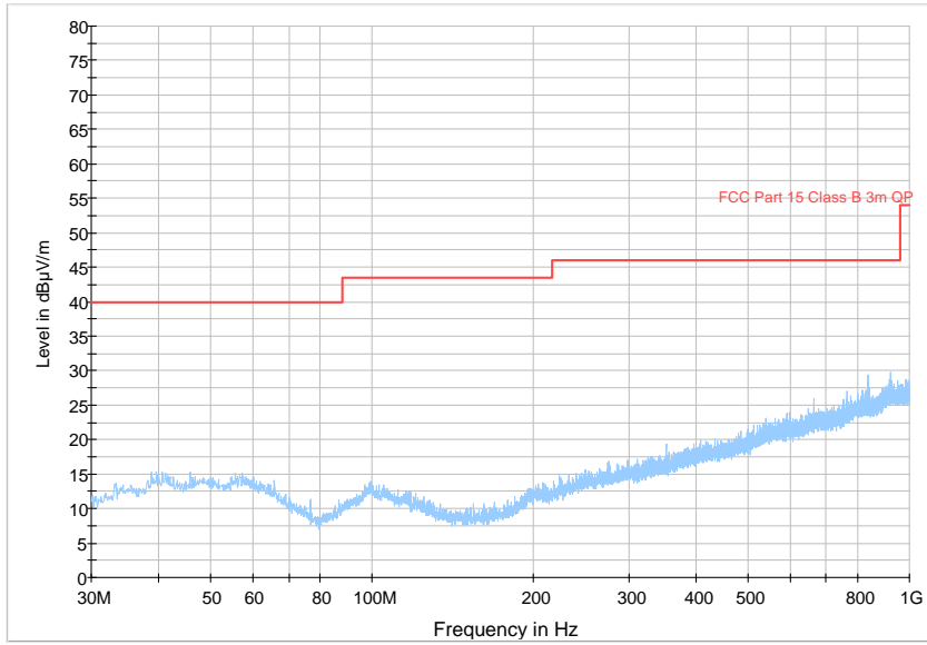
Radiated Emissions 30 - 1000 MHz, GFSK
