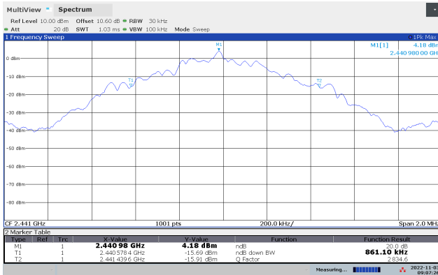
20dB Bandwidth 2441 MHz, GFSK
