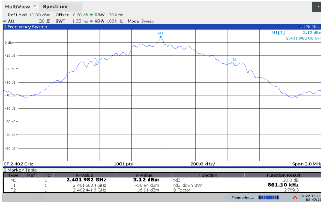
20dB Bandwidth 2402 MHz, GFSK
