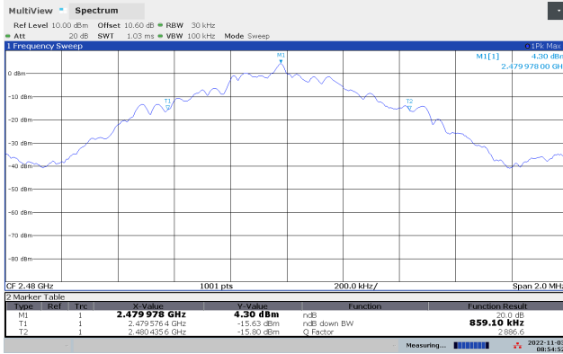
20dB Bandwidth 2480 MHz, GFSK
