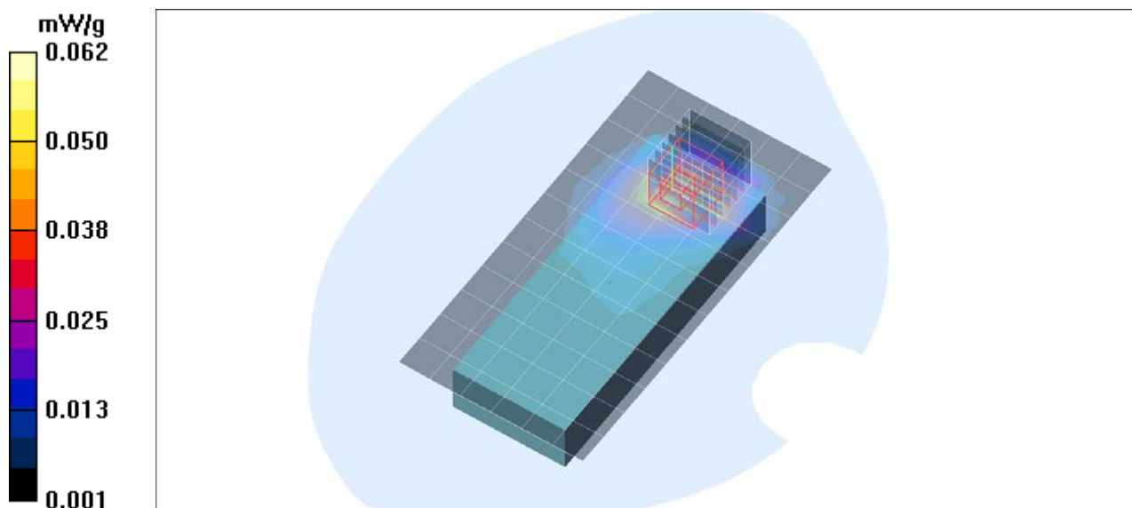
Plot. 2: SAR distribution plot for DECT, channel 0, body worn configuration, front side, 0 mm to phantom.
