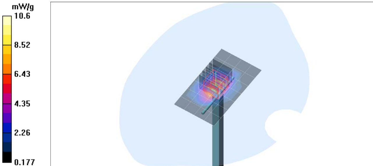
Plot. 3: SAR Verification Measurement 1900 MHz (December 05, 2022).
