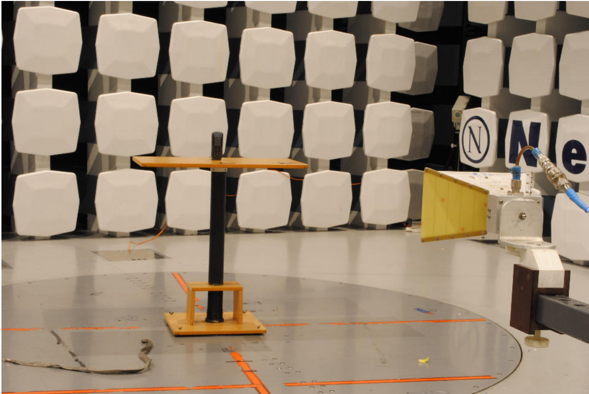
Radiated Tests
