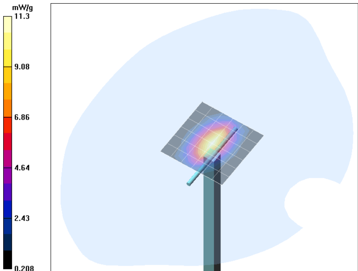
Fig. 12: Validation measurement 1900 MHz body (May 19, 2008), coarse grid. Ambient Temperature: 22.7° C, Liquid Temperature: 21.8° C.
