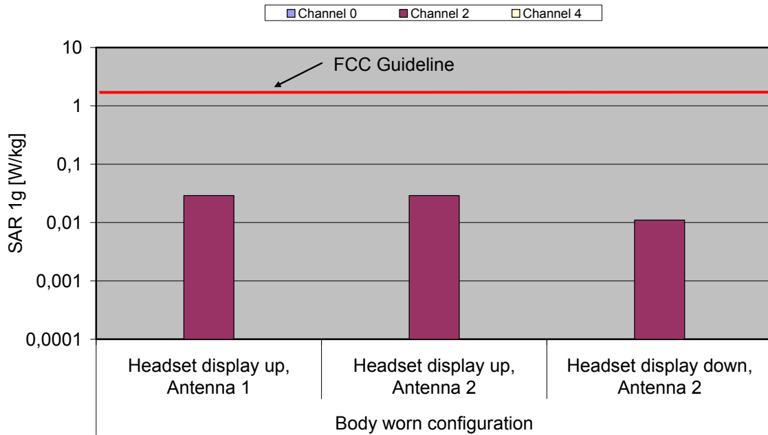
Fig. 10: The measured SAR values in body-worn configuration for the Ascom DH4 for the US DECT standard in comparison to the FCC exposure limit.
