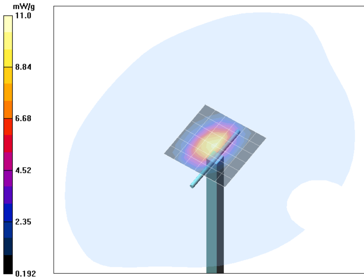
Fig. 11: Validation measurement 1900 MHz Head (May 15, 2008), coarse grid. Ambient Temperature: 23.1° C, Liquid Temperature: 21.9° C.
