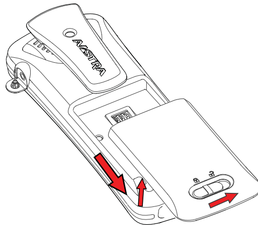
Figure 8. Easy replaceable battery, unlock the lid and remove the battery.
