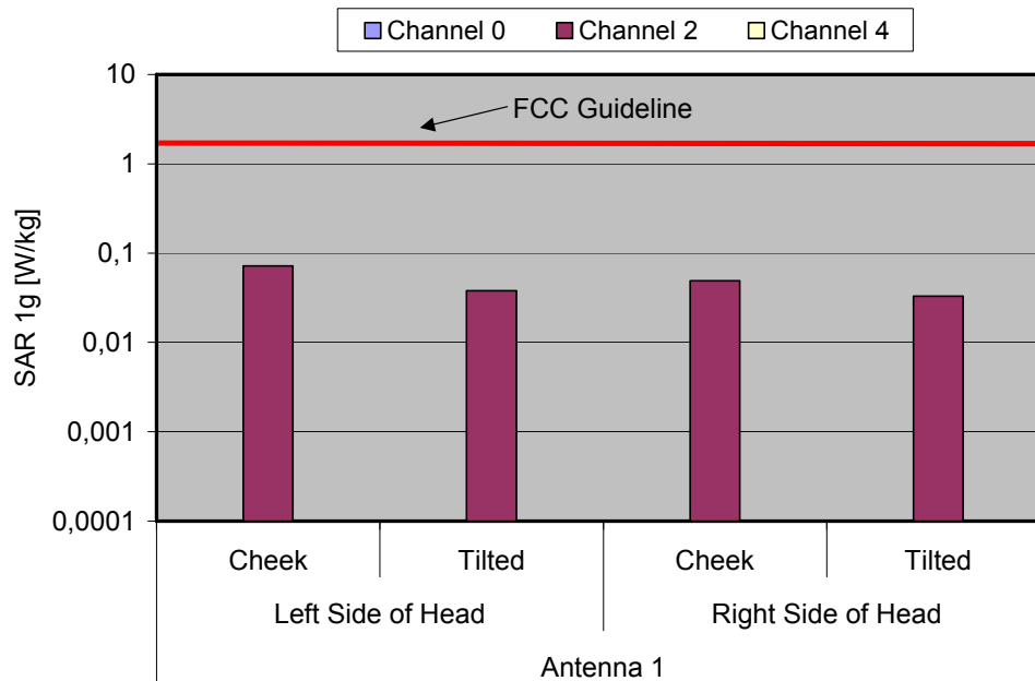
Fig. 8: The measured head phantom SAR values for the Ascom DH4, with antenna 1 for the US DECT standard in comparison to the FCC exposure limit.
