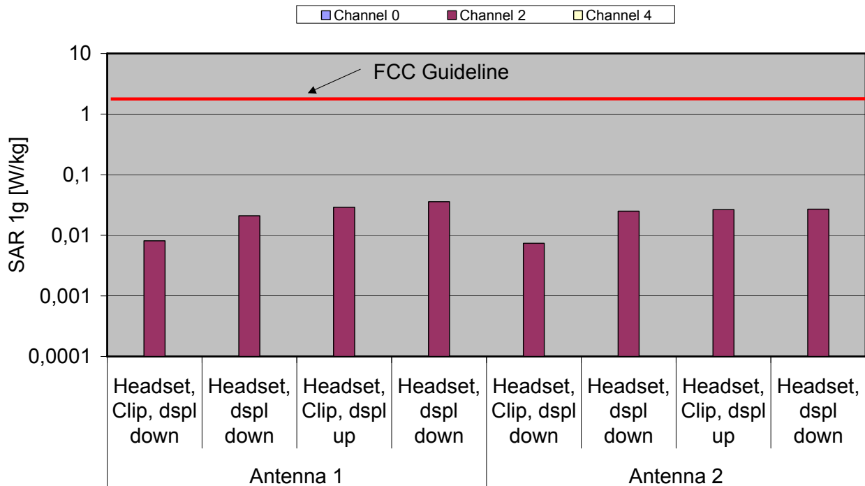
Fig. 10: The measured SAR values in body-worn configuration for the Ascom DH4 for the US DECT standard in comparison to the FCC exposure limit.
