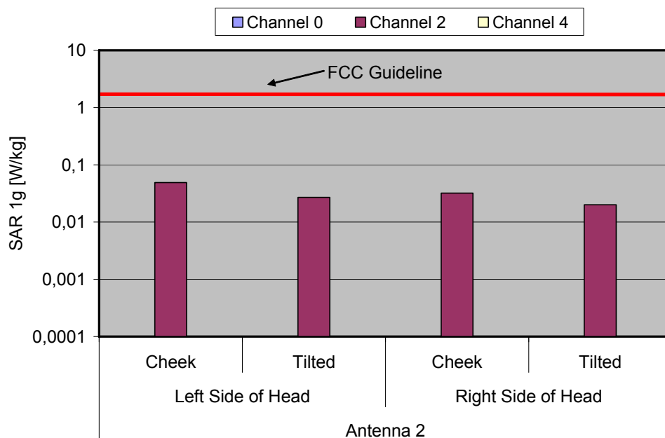
Fig. 9: The measured head phantom SAR values for the Ascom DH4, with antenna 2 for the US DECT standard in comparison to the FCC exposure limit.
