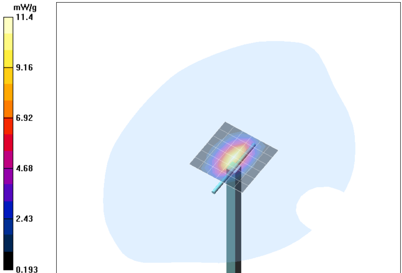
Fig. 12: Validation measurement 1900 MHz body (September 09, 2008), coarse grid. Ambient Temperature: 22.6° C, Liquid Temperature: 21.5° C.
