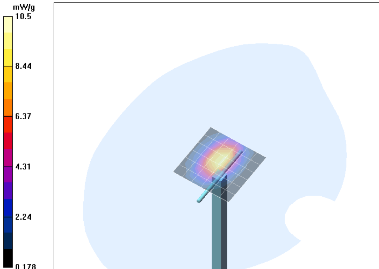
Fig. 11: Validation measurement 1900 MHz Head (September 08, 2008), coarse grid. Ambient Temperature: 22.8° C, Liquid Temperature: 21.6° C.
