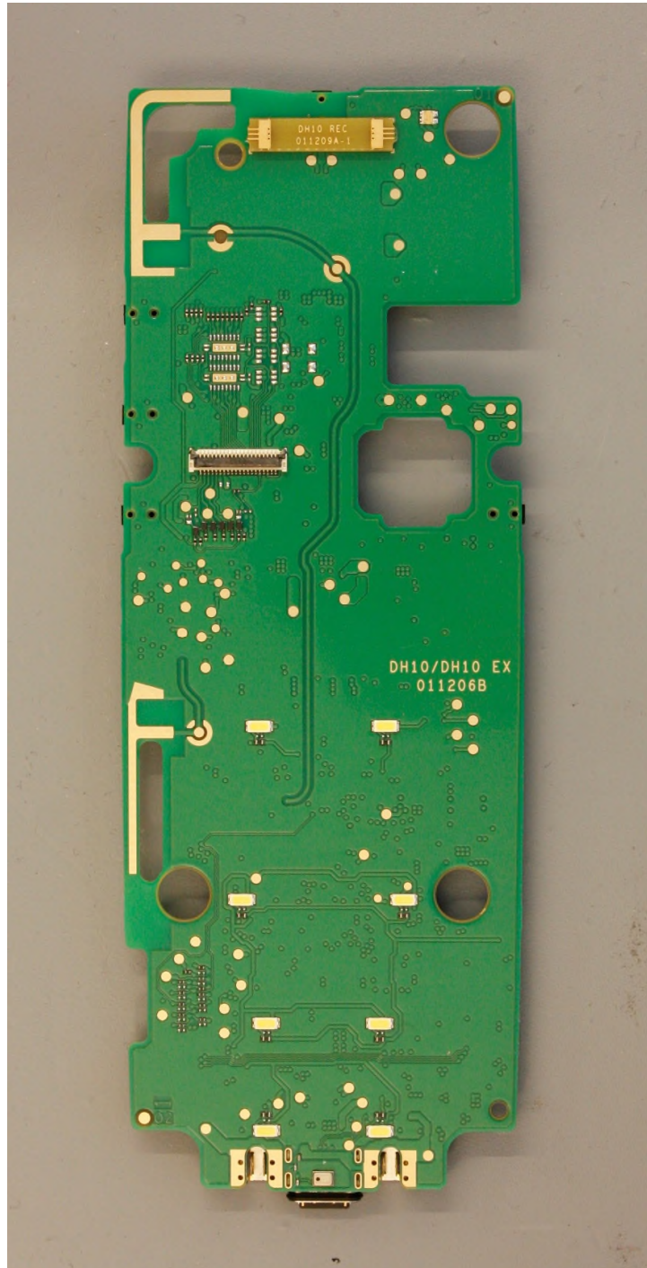
Figure 9: Main PCBA front side
