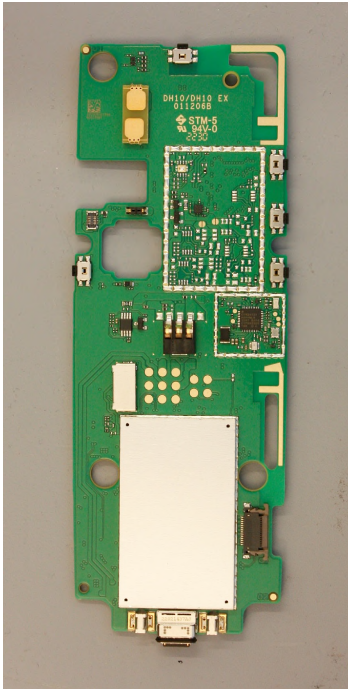
Figure 10: Main PCB back side
