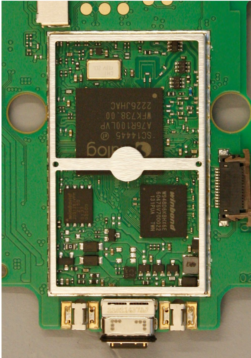
Figure 11: Shield can, back side
