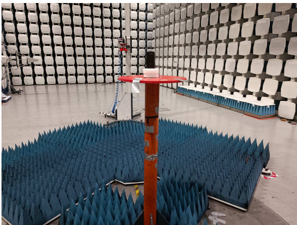
Radiated Emissions above 1 GHz (FCC Part 15C)
