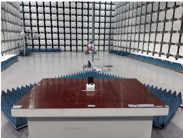
Radiated Emissions above 1 GHz (FCC Part 15B)
