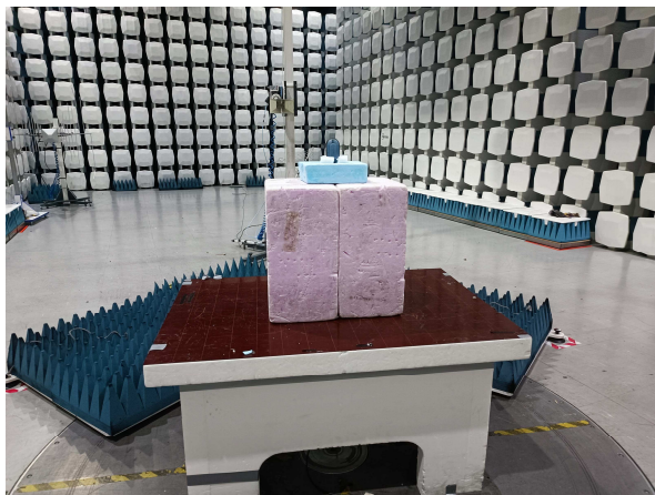
Radiated Emissions 1 – 5 GHz
