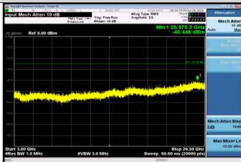
Band41-5MHz-16QAM-39675-1RB#0-Range3:3000~26500MHz
