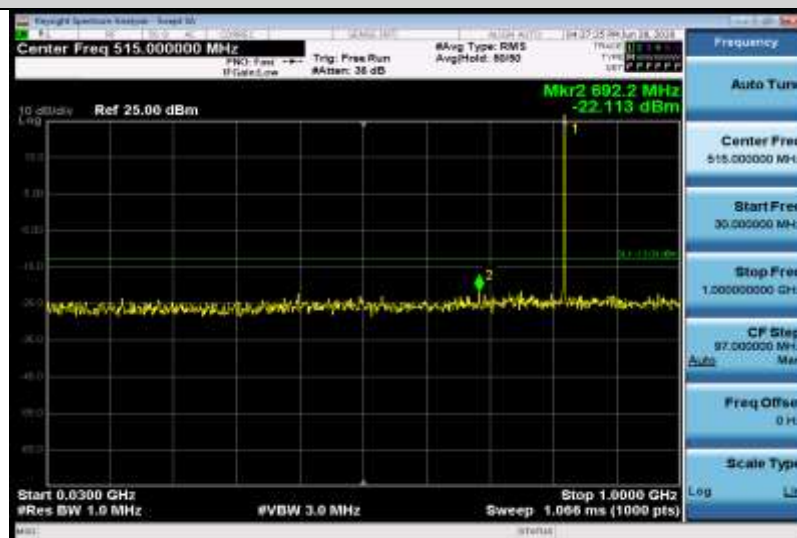
Band26-1.4MHz-QPSK-26783-1RB#0-Range1:30~1000MHz
