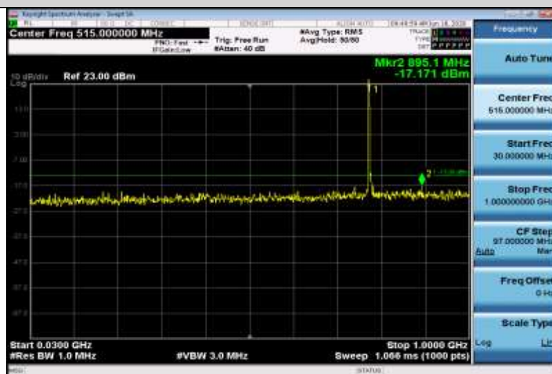
Band13-10MHz-16QAM-23230-1RB#0-Range1:30~1000MHz
