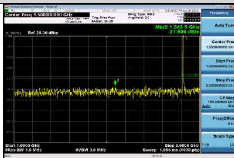
Band25-5MHz-QPSK-26665-1RB#0-Range2:1000~2000MHz
