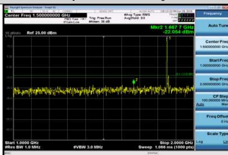
Band25-10MHz-16QAM-26090-1RB#0-Range2:1000~2000MHz
