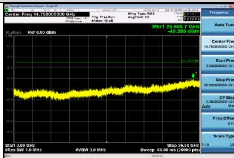
Band41-20MHz-QPSK-40620-1RB#0-Range3:3000~26500MHz
