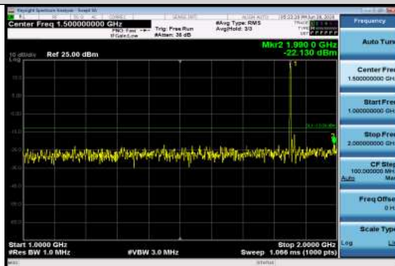
Band25-15MHz-16QAM-26115-1RB#0-Range2:1000~2000MHz
