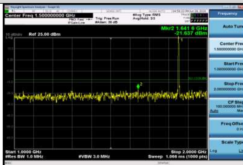
Band25-3MHz-16QAM-26055-1RB#0-Range2:1000~2000MHz
