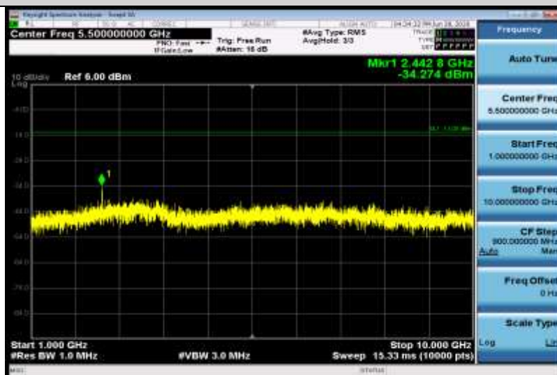
Band26-5MHz-16QAM-26715-1RB#0-Range2:1000~10000MHz
