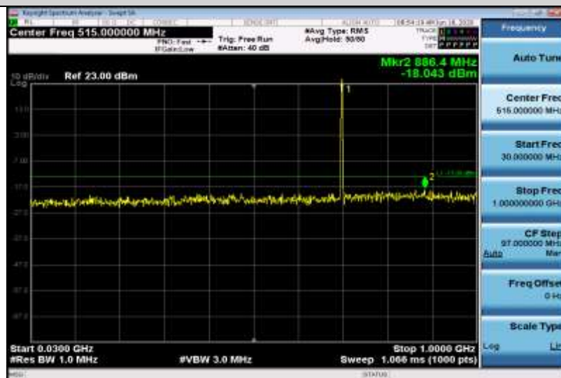
Band12-5MHz-16QAM-23095-1RB#0-Range1:30~1000MHz
