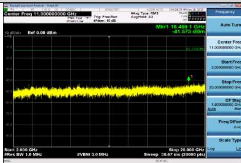
Band4-1.4MHz-QPSK-20175-1RB#0-Range3:2000~20000MHz
