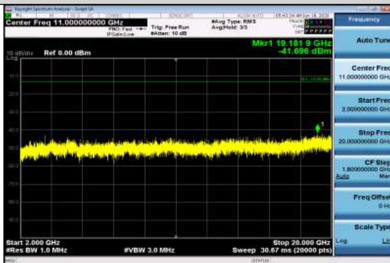
Band4-15MHz-16QAM-20025-1RB#0-Range3:2000~20000MHz
