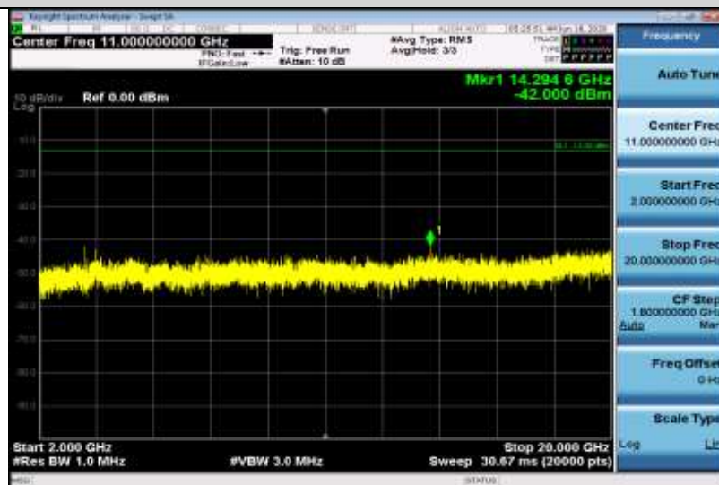
Band4-10MHz-16QAM-20175-1RB#0-Range3:2000~20000MHz
