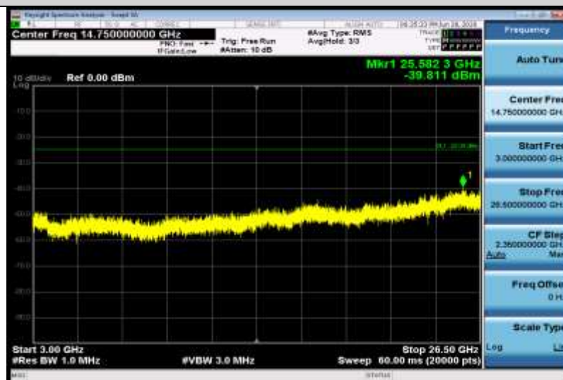
Band7-15MHz-QPSK-20825-1RB#0-Range3:3000~26500MHz
