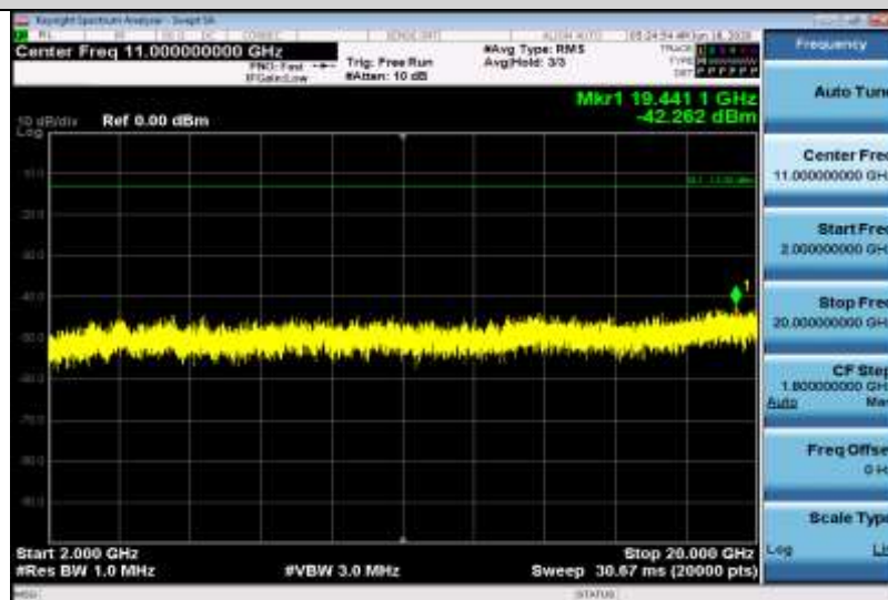
Band4-10MHz-16QAM-20000-1RB#0-Range3:2000~20000MHz
