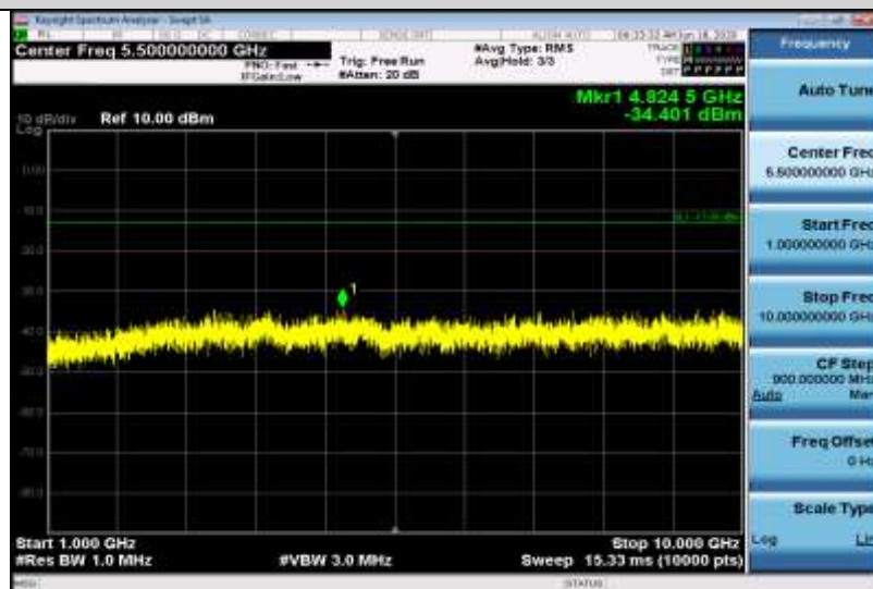
Band5-1.4MHz-QPSK-20643-1RB#0-Range2:1000~10000MHz
