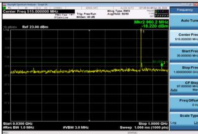
Band5-10MHz-16QAM-20525-1RB#0-Range1:30~1000MHz
