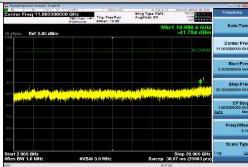
Band4-20MHz-16QAM-20050-1RB#0-Range3:2000~20000MHz
