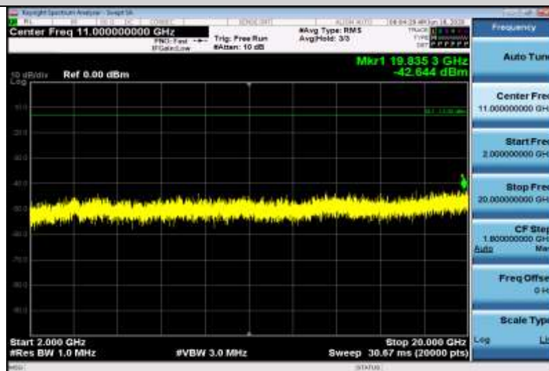
Band4-20MHz-QPSK-20300-1RB#0-Range3:2000~20000MHz
