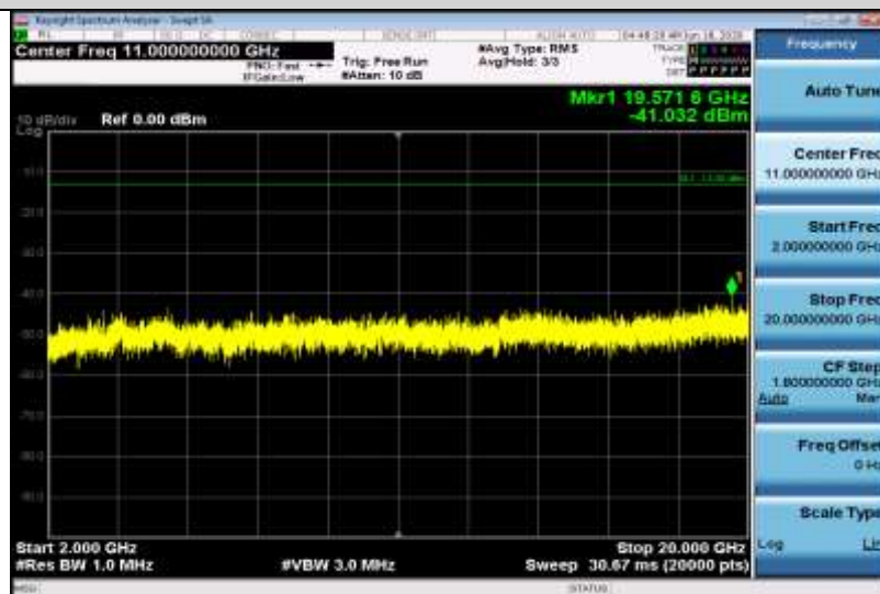
Band4-3MHz-16QAM-19965-1RB#0-Range3:2000~20000MHz
