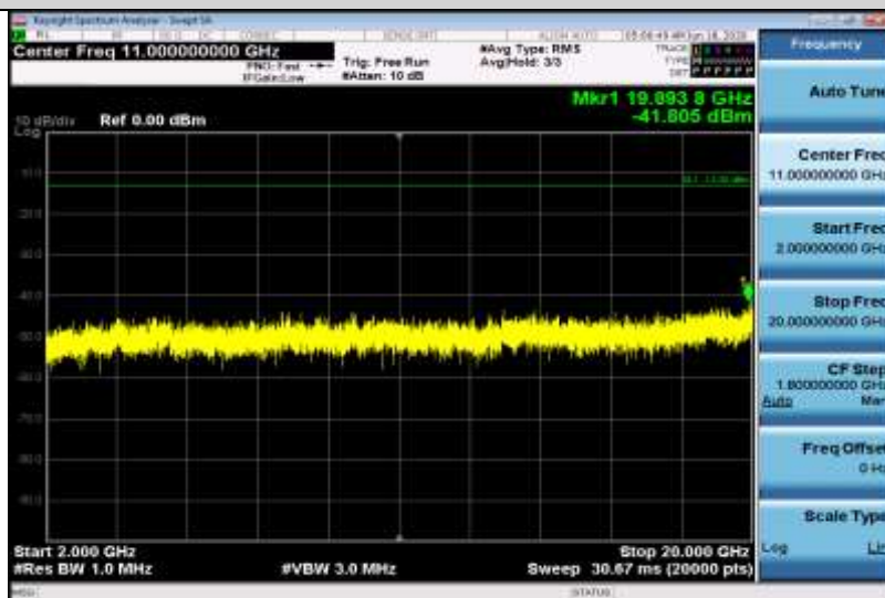
Band4-5MHz-16QAM-19975-1RB#0-Range3:2000~20000MHz
