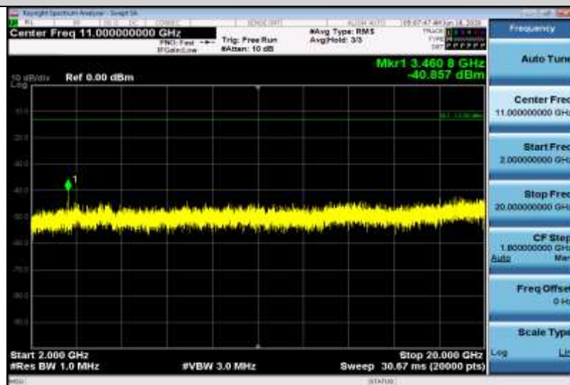
Band4-5MHz-16QAM-20175-1RB#0-Range3:2000~20000MHz
