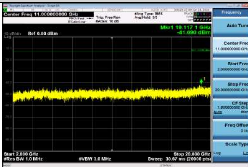
Band4-10MHz-QPSK-20175-1RB#0-Range3:2000~20000MHz
