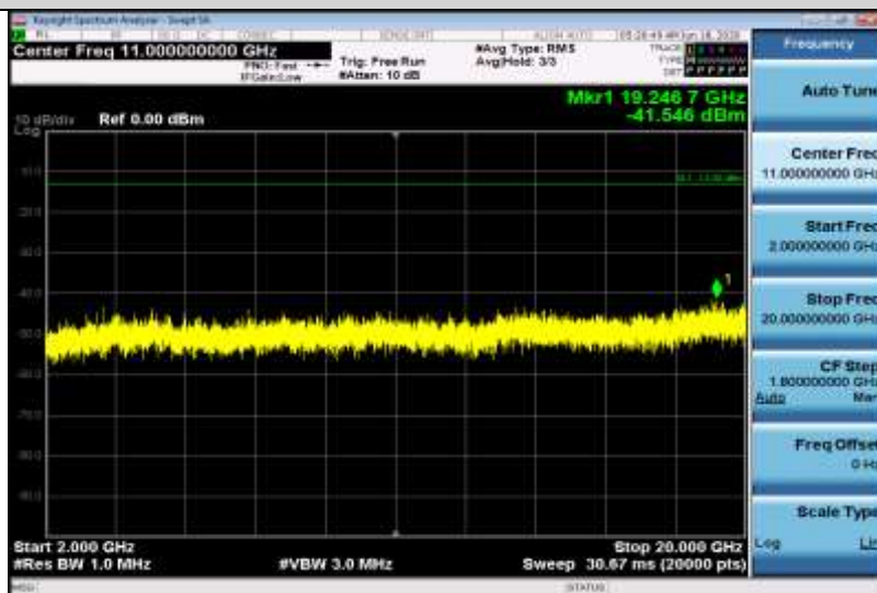
Band4-10MHz-16QAM-20350-1RB#0-Range3:2000~20000MHz
