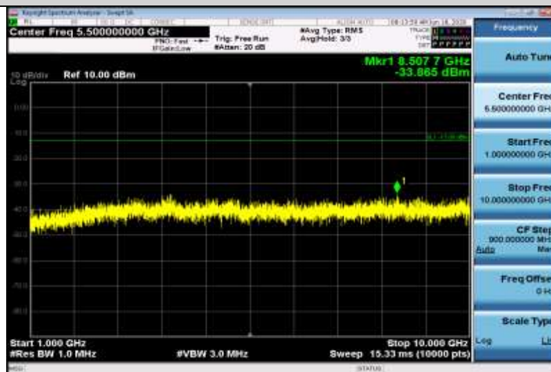
Band12-1.4MHz-16QAM-23173-1RB#0-Range2:1000~10000MHz
