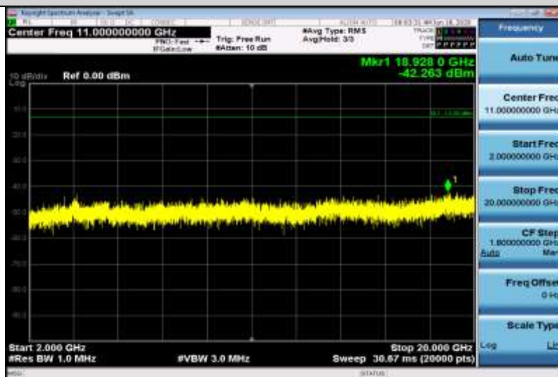
Band4-20MHz-QPSK-20175-1RB#0-Range3:2000~20000MHz
