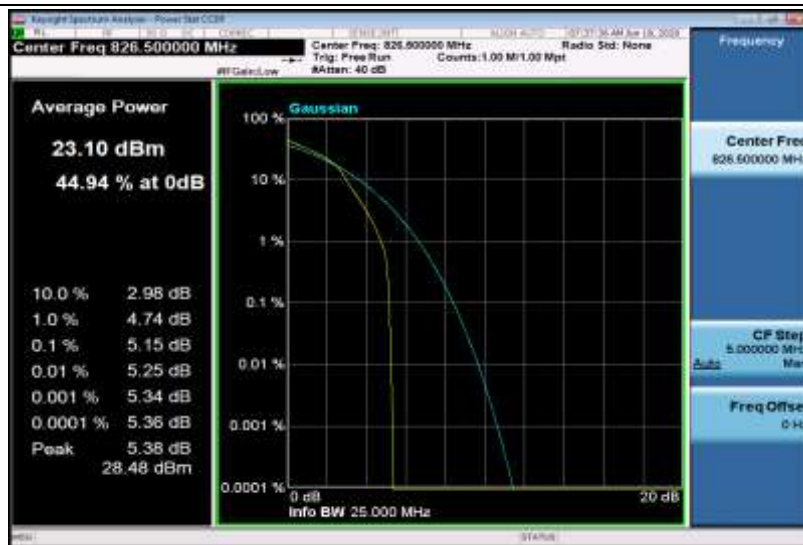
Band5-5MHz-16QAM-20425-25RB#0
