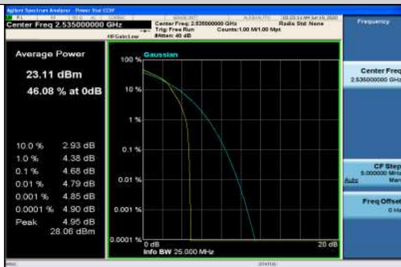
Band7-10MHz-16QAM-21100-50RB#0
