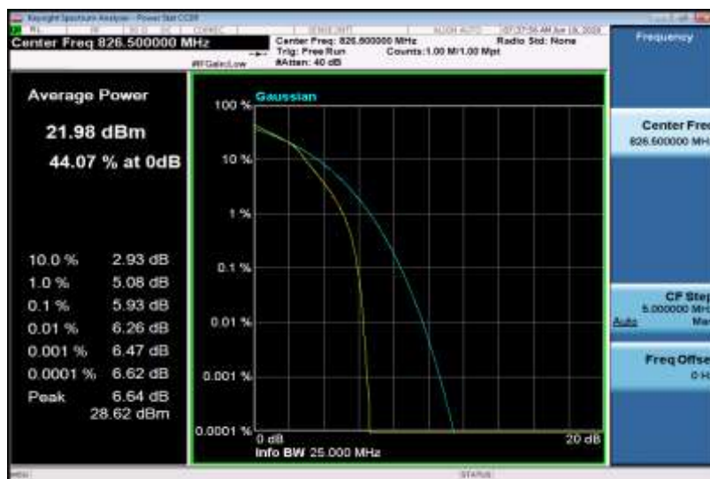
Band5-5MHz-16QAM-20525-1RB#0
