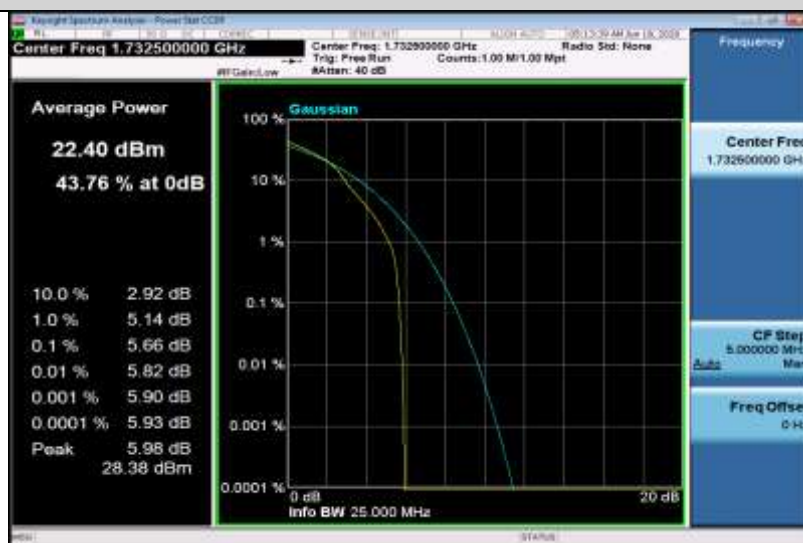
Band4-5MHz-16QAM-20175-25RB#0
