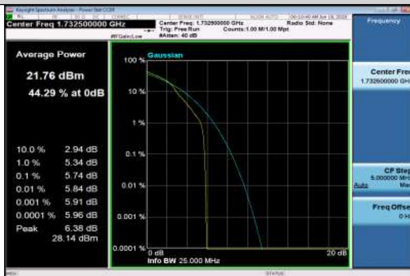
Band4-20MHz-16QAM-20175-100RB#0
