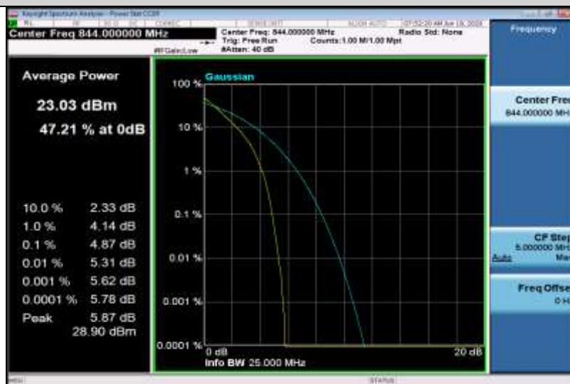
Band5-10MHz-16QAM-20450-1RB#0
