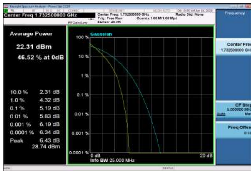
Band4-20MHz-QPSK-20300-1RB#0
