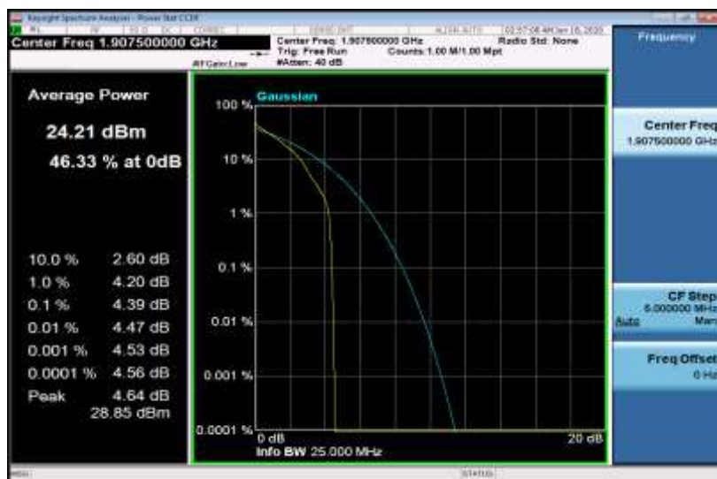
Band2-5MHz-QPSK-19175-25RB#0
