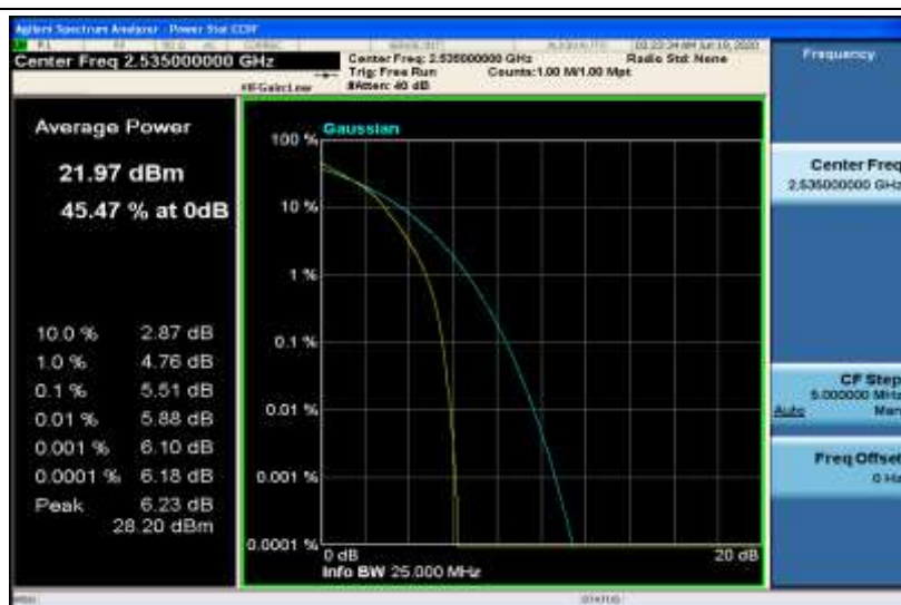
Band7-10MHz-16QAM-21400-1RB#0
