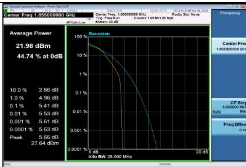
Band2-10MHz-16QAM-18650-50RB#0
