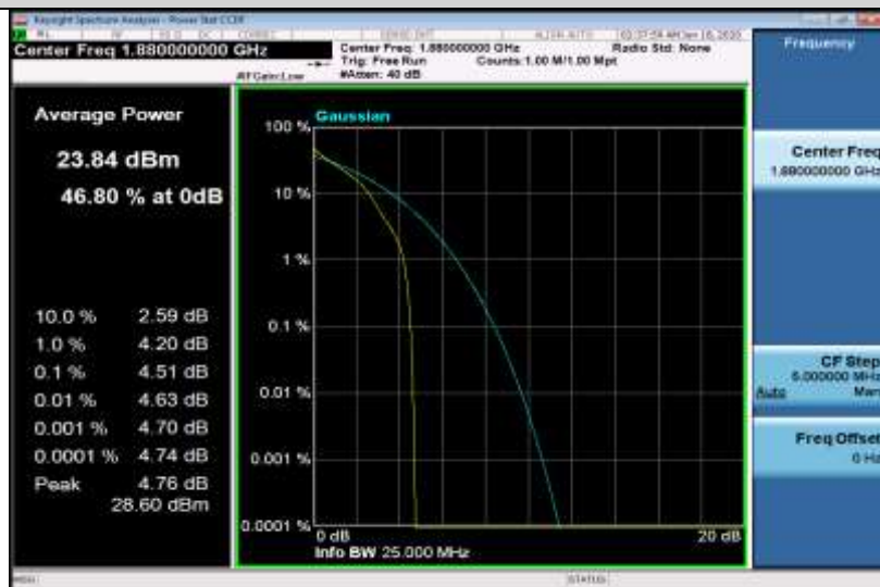
Band2-3MHz-QPSK-18900-15RB#0
