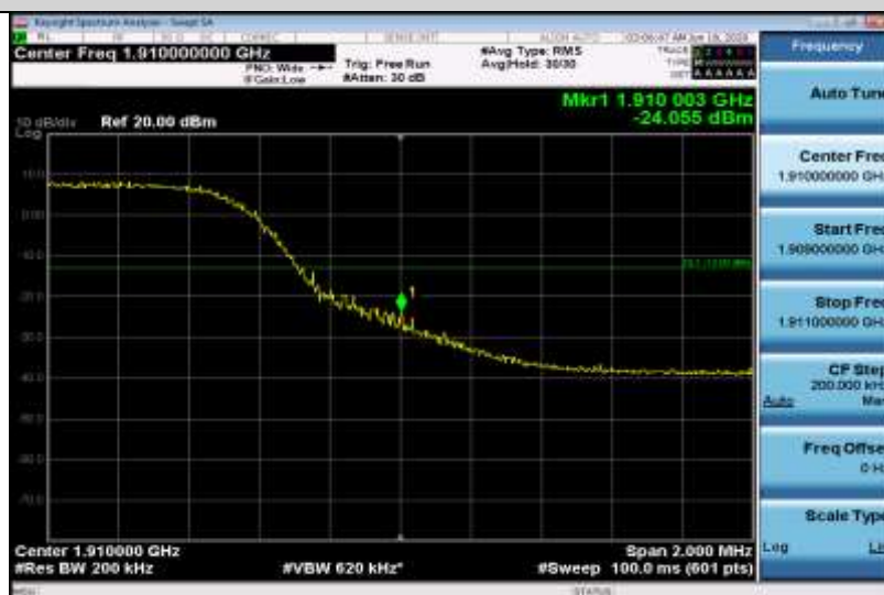
Band2-10MHz-16QAM-18650-1RB#49
