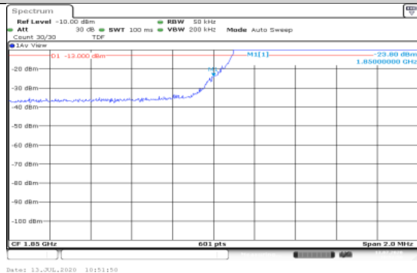
Band2-3MHz-16QAM-19185-1RB#0
