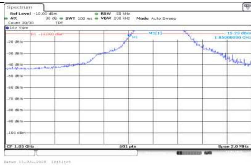
Band2-3MHz-16QAM-18615-1RB#14
