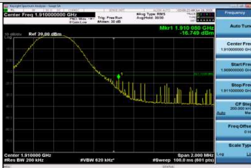
Band2-10MHz-QPSK-19150-1RB#49
