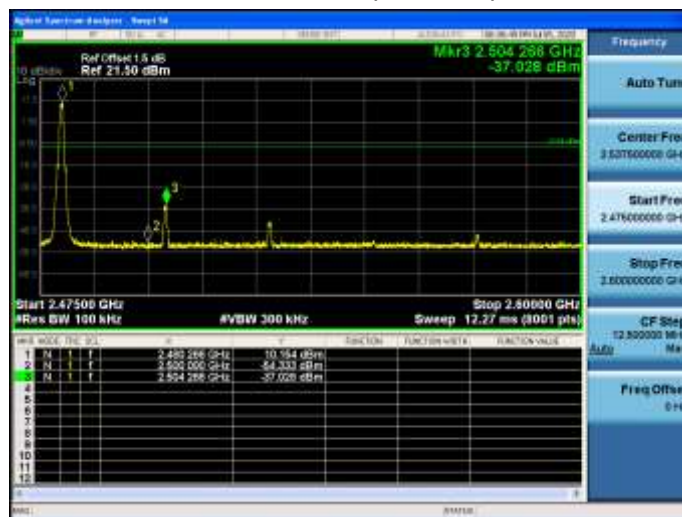
Mode 1 CH39(2480MHz)
