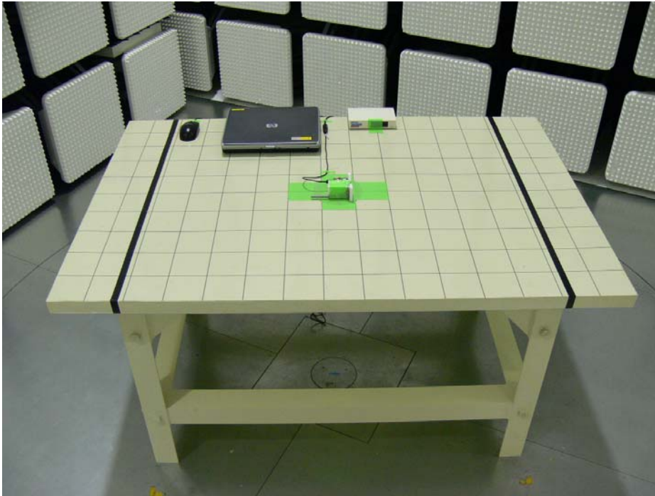
Photograph 8: Set-up for Radiated Emission of Transmitter external antenna, Front View
