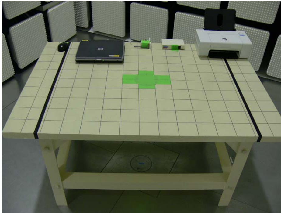
Photograph 10: Set-up for Radiated Emission of Receiver, Front View
