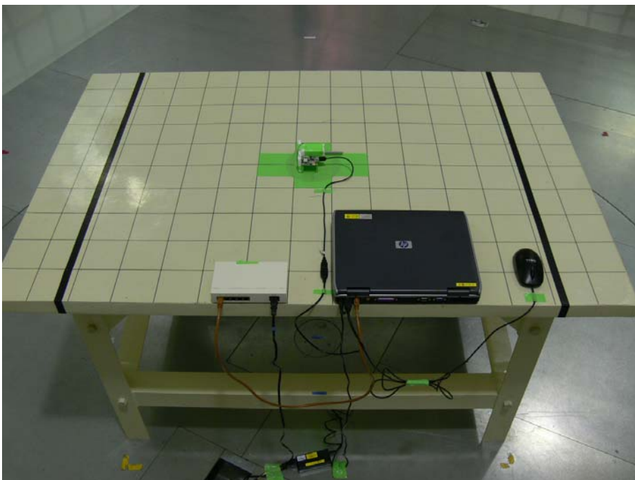
Photograph 9: Set-up for Radiated Emission of Transmitter external antenna, Rear View
