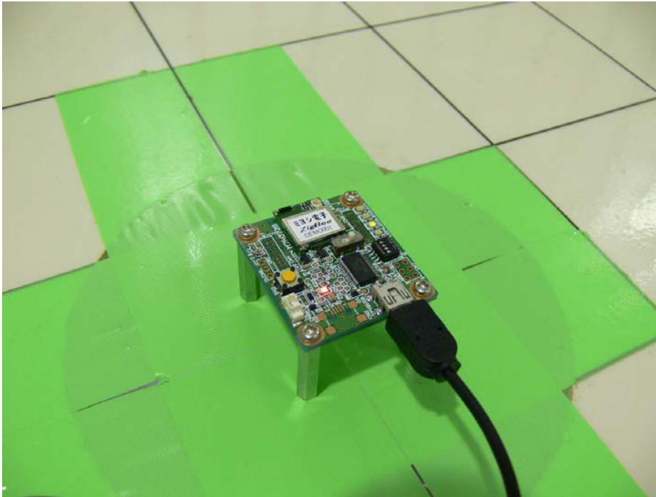
Photograph 15: Set-up for Radiated Emission, EUT Configuration internal antenna X-Axis
