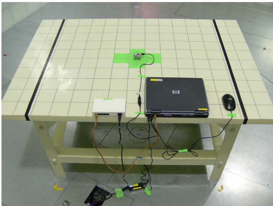
Photograph 7: Set-up for Radiated Emission of Transmitter internal antenna, Rear View
