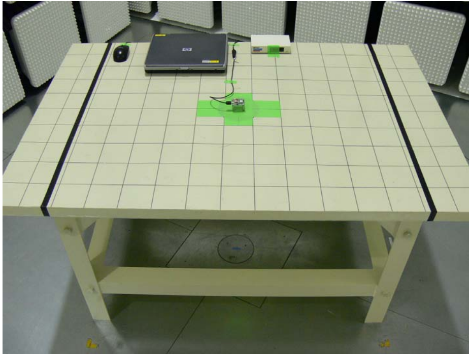
Photograph 6: Set-up for Radiated Emission of Transmitter internal antenna, Front View
