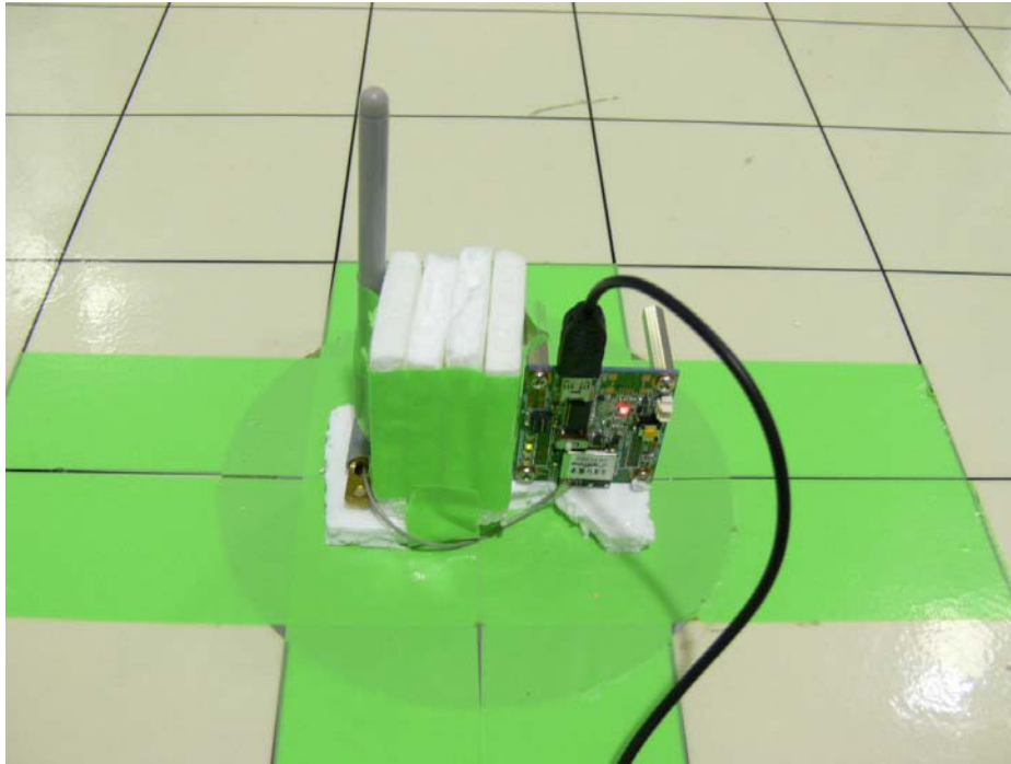
Photograph 14: Set-up for Radiated Emission, EUT Configuration external antenna Z-Axis
