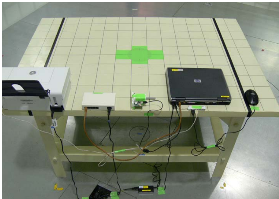
Photograph 11: Set-up for Radiated Emission of Receiver, Rear View
