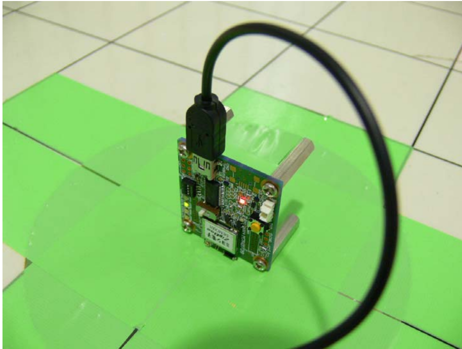
Photograph 17: Set-up for Radiated Emission, EUT Configuration internal antenna Z-Axis
