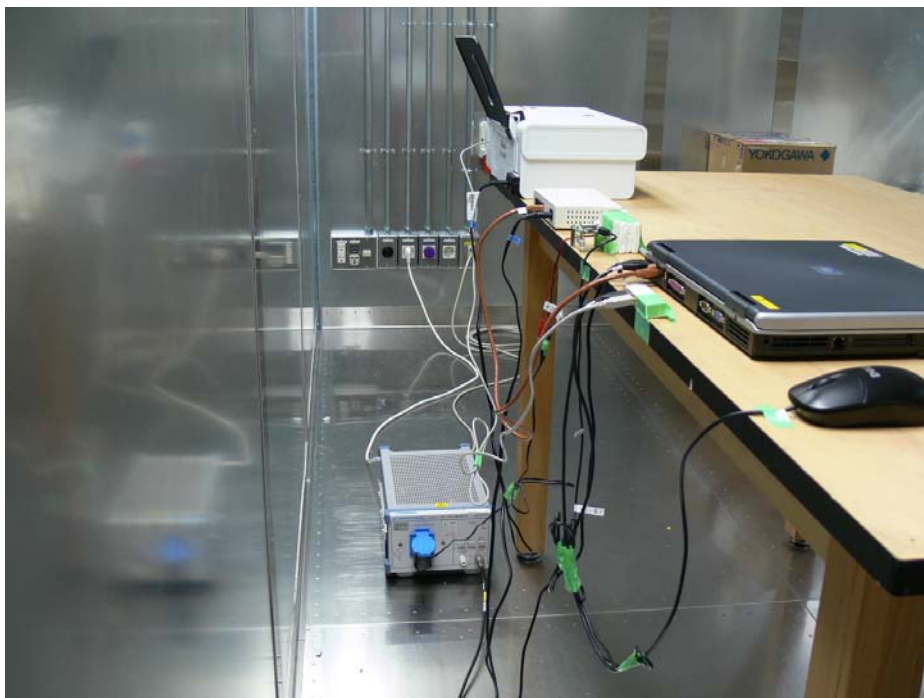
Photograph 5: Set-up for AC Power Line Conducted Emission of Receiver, Rear View
