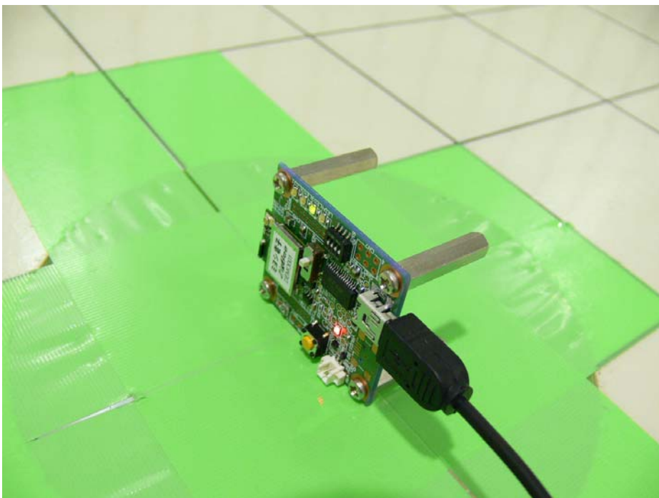
Photograph 16: Set-up for Radiated Emission, EUT Configuration internal antenna Y-Axis
