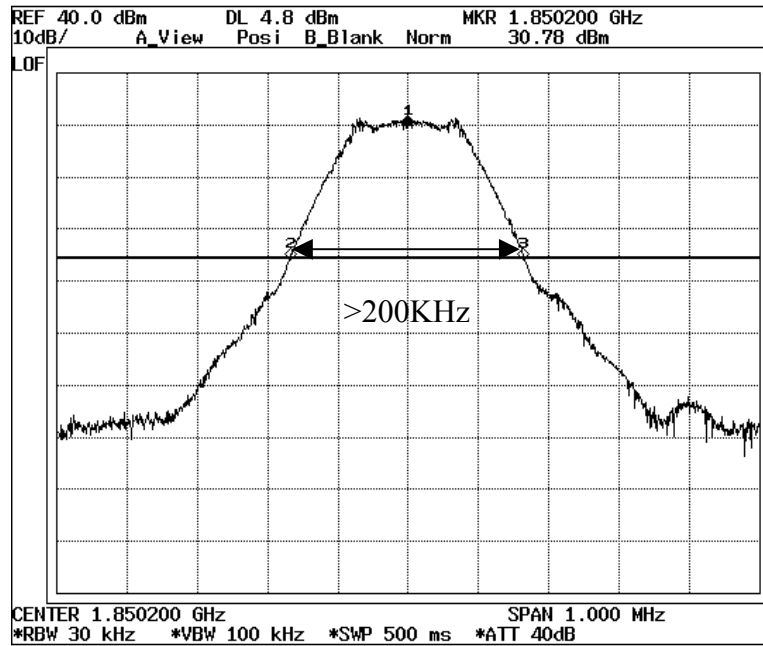
Circuit Switched (GSM Mode CH512)
