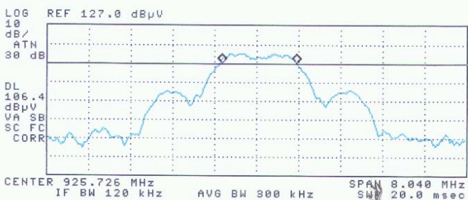
PLOT 3 BASE STATION 6dB BANDWIDTH Channel 20
