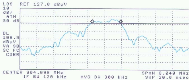
PLOT 1 BASE STATION 6dB BANDWIDTH Channel 1
