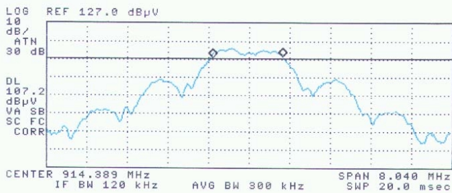
PLOT 2 BASE STATION 6dB BANDWIDTH Channel 2
