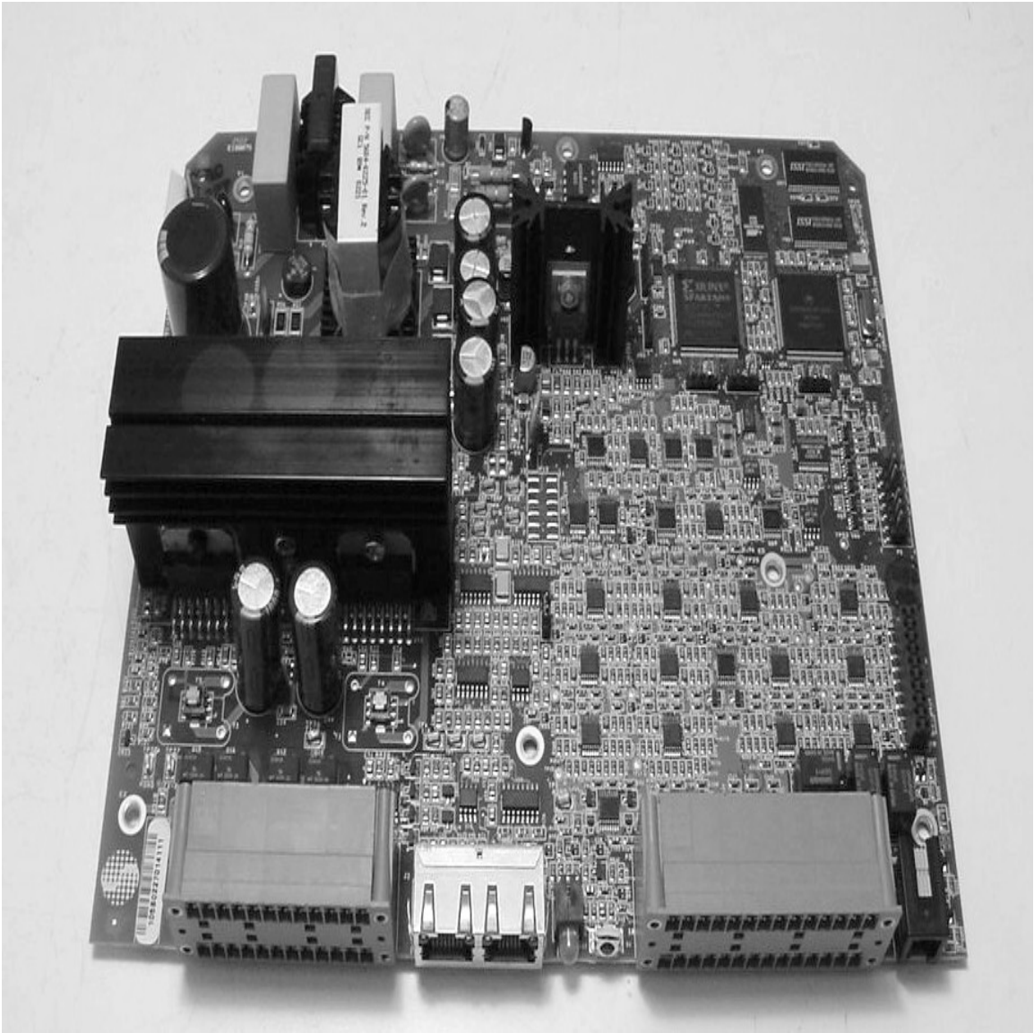
Controller Printed Circuit Board Assembly, Top View
