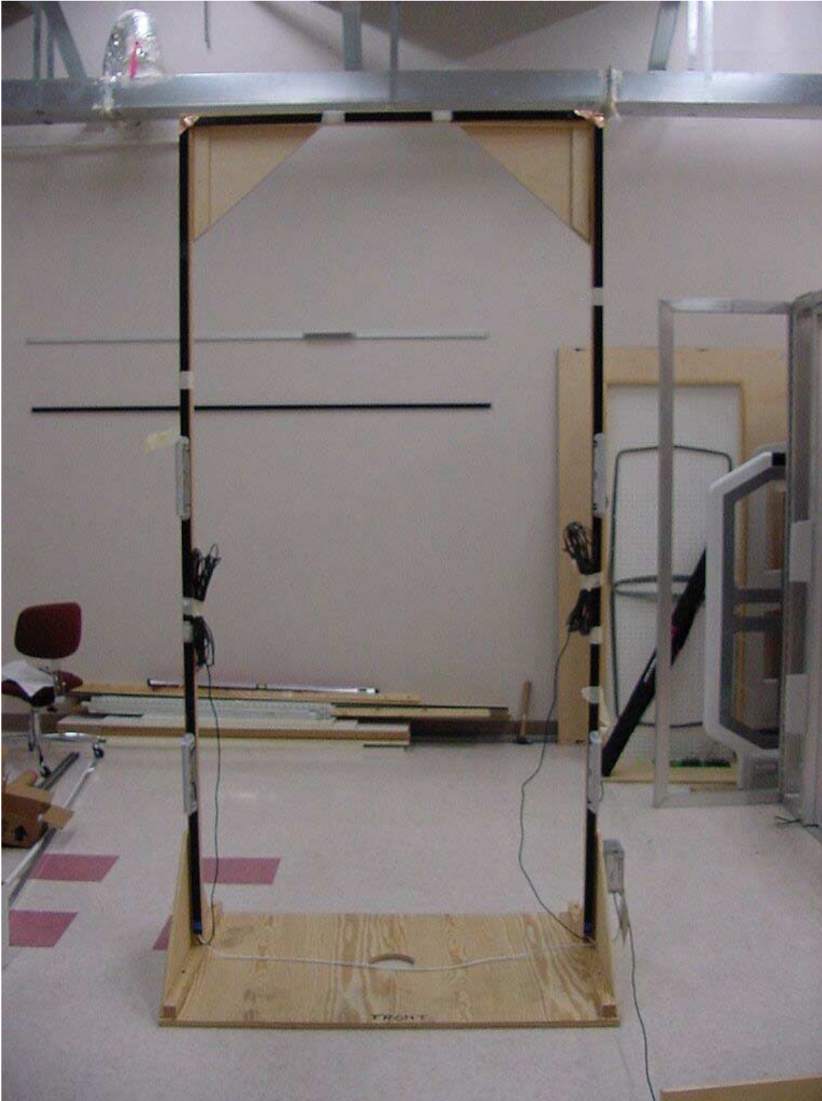
Figure 2: Loop system 2 – antenna assembly (120x244cm small loop) for emission tests. For H field test 200x244x60cm fig.8 loop was used..
