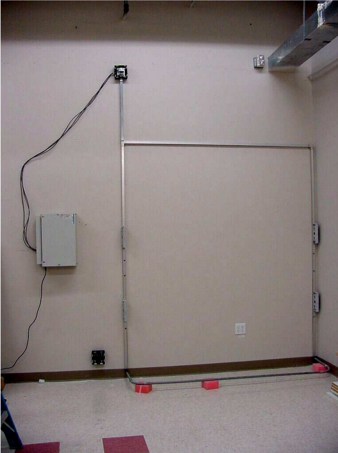
Figure 1: Loop system 1 – full assembly for safety test. Tx coil inside an aluminum extrusion.
