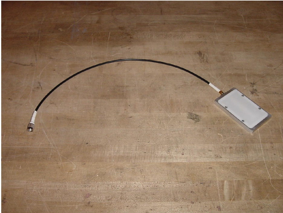
Photo of Near Field Antenna and Cable
