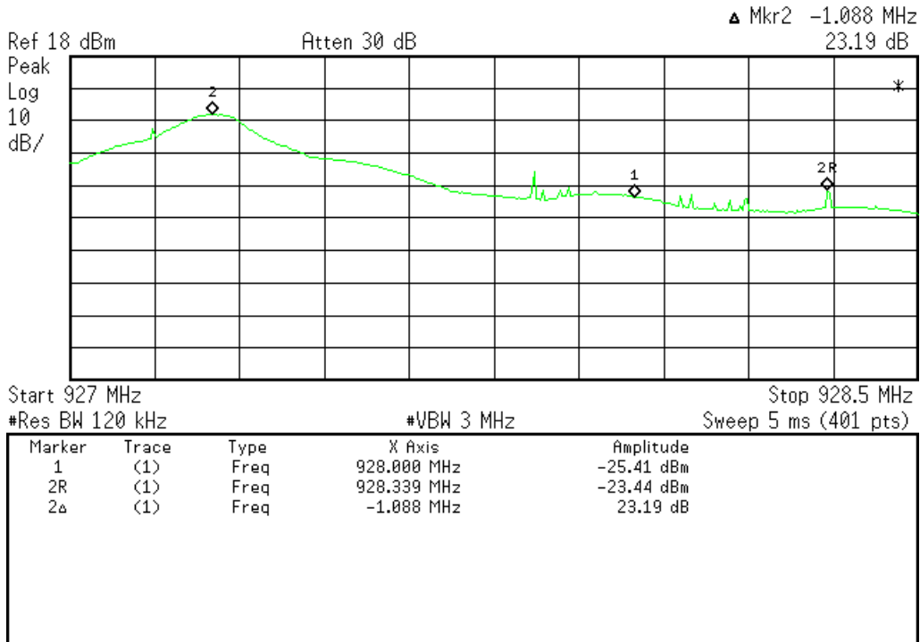
Band Edge High End (Hopping disabled)
