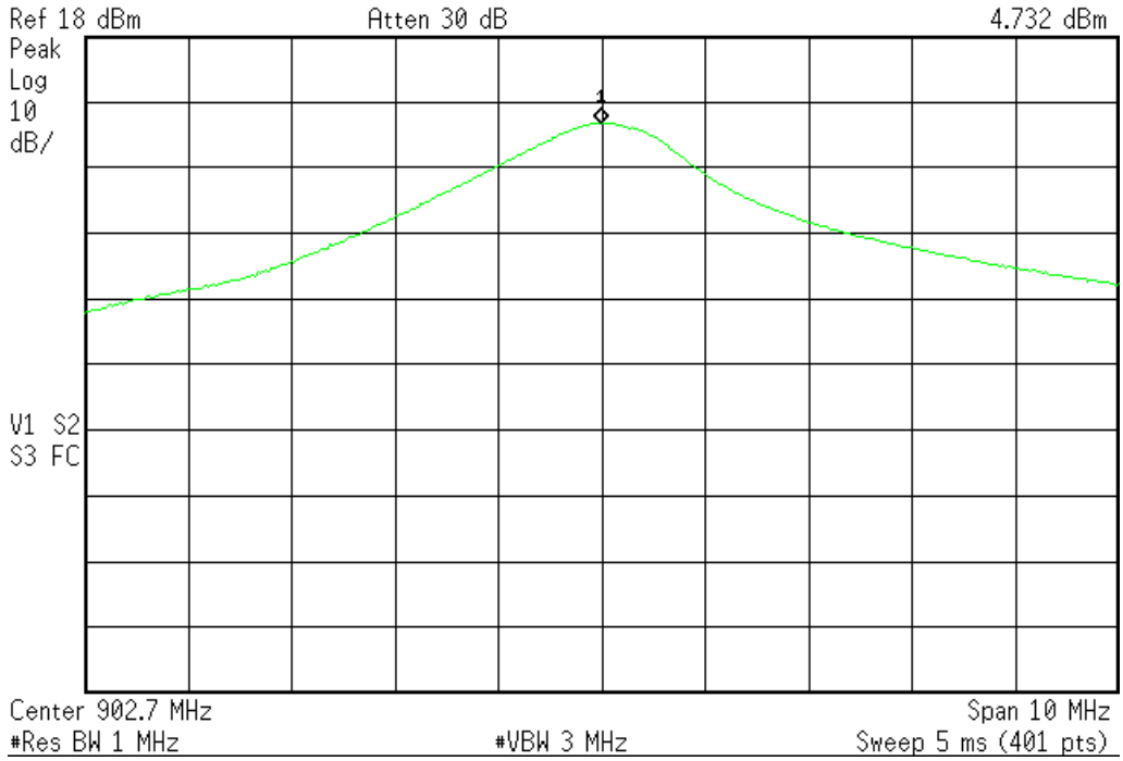
Peak output power UHF Antenna Port 2, Channel 0
