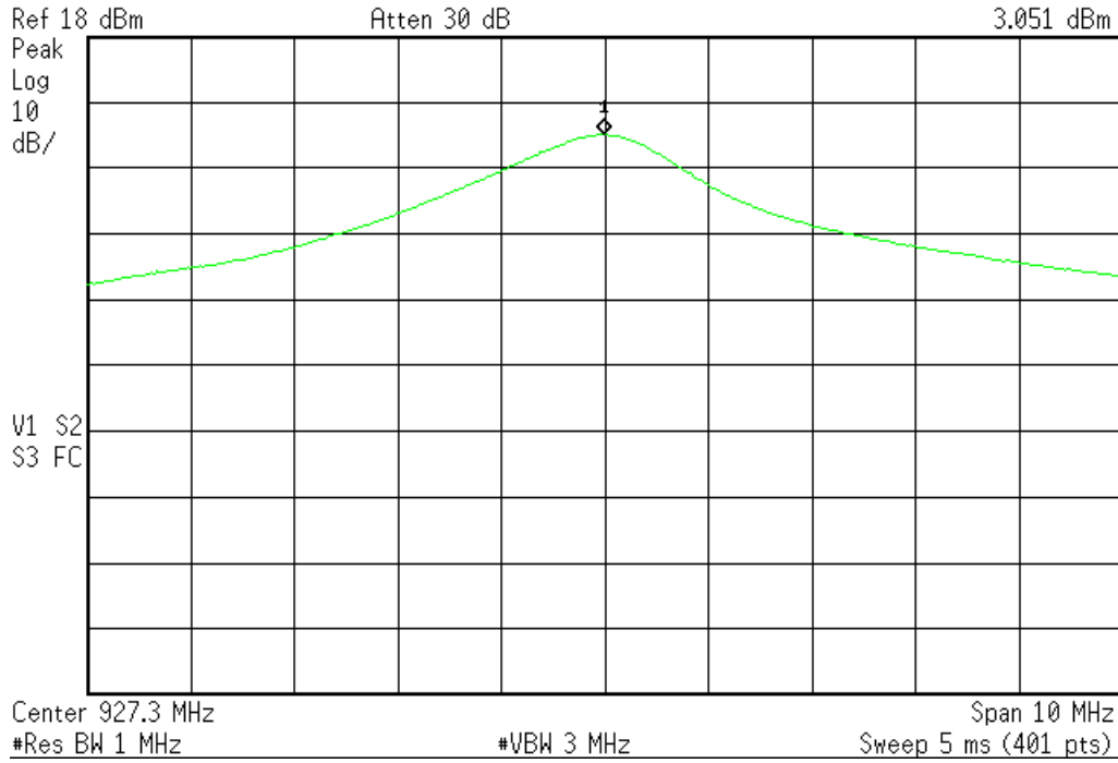
Peak output power UHF Antenna Port 2, Channel 49
