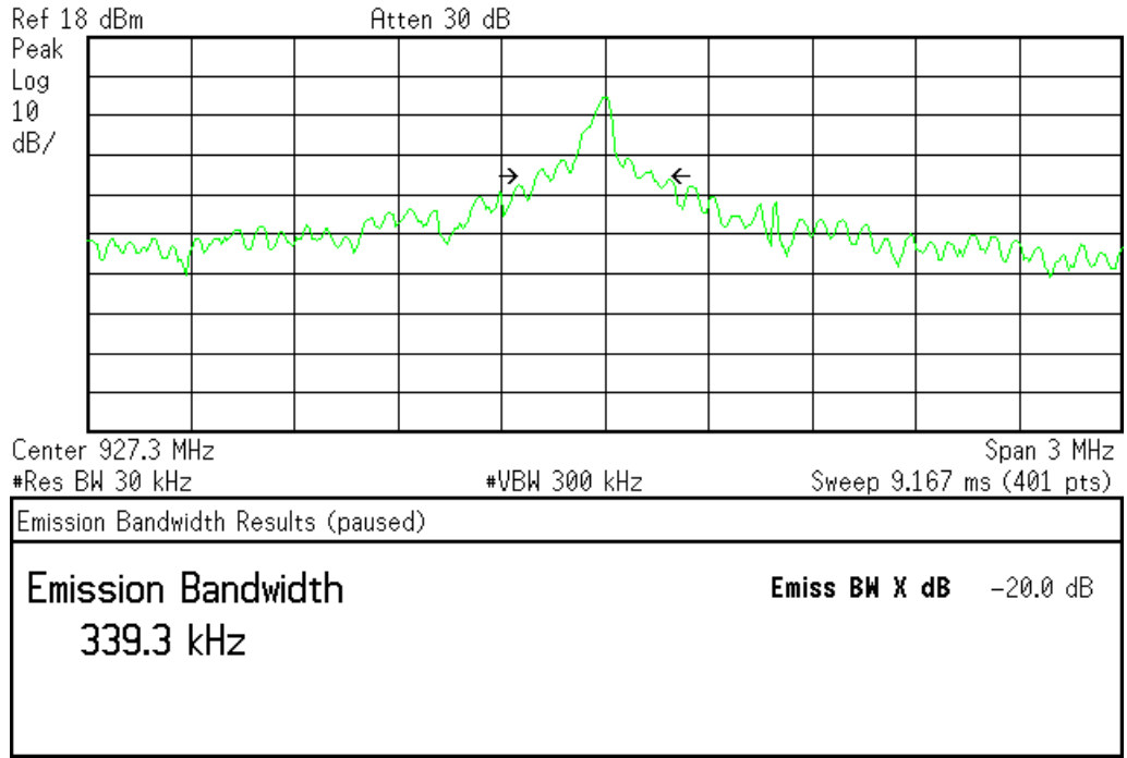
20dB bandwidth channel 49 UHF Antenna Port 1
