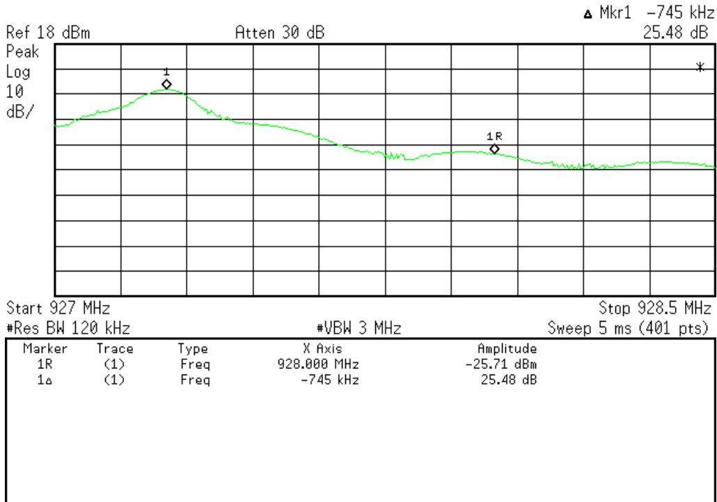
Band Edge High End (Hopping enabled)
