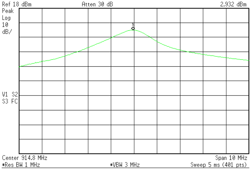
Peak output power UHF Antenna Port 1, Channel 24
