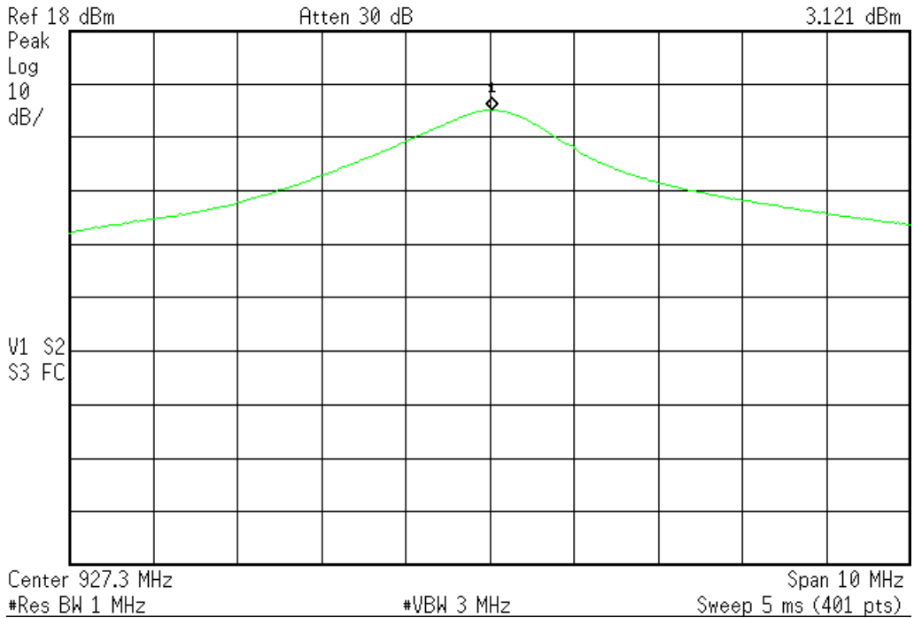
Peak output power UHF Antenna Port 1, Channel 49
