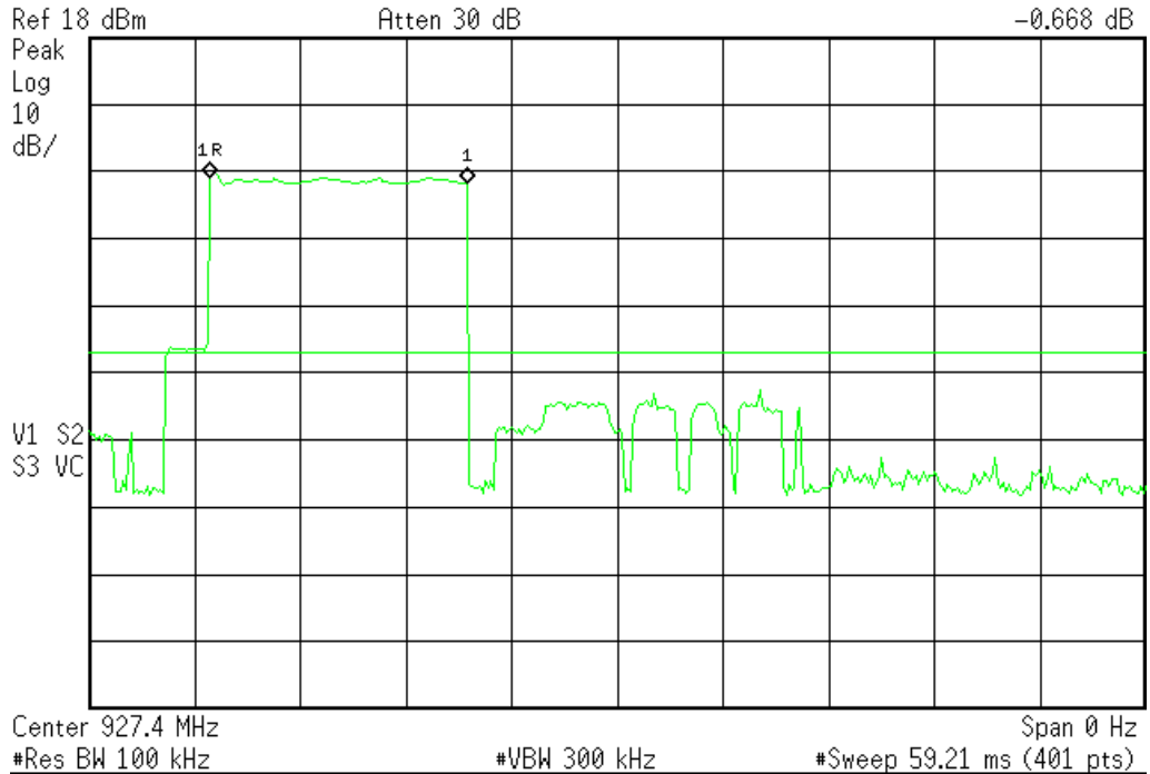
UHF Antenna Port 1, CH 49, Time of Occupancy (plot2)
