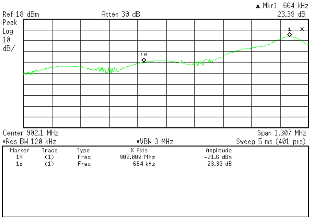
Band Edge Low End (Hopping enabled)
