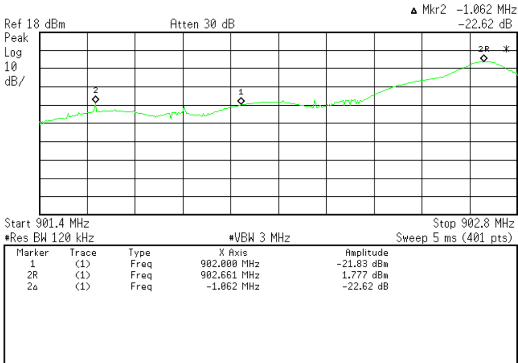
Band Edge Low End (Hopping disabled)
