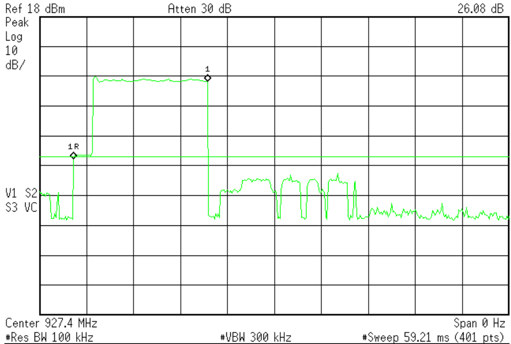
UHF Antenna Port 1, CH 49, Time of Occupancy (plot1)
