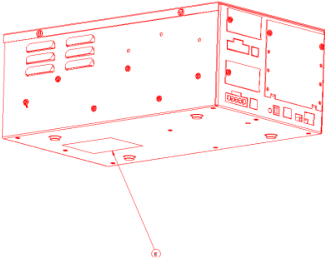
Scan Thru Platform, Bottom View – Compliance Label, containing FCC label requirements.
