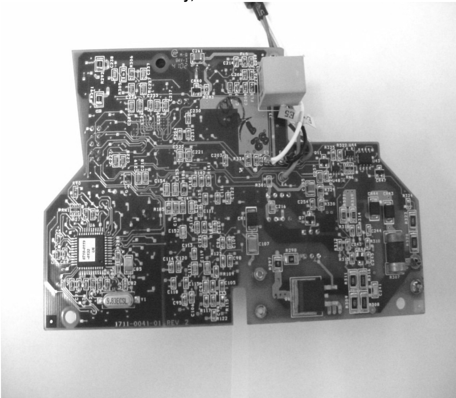
Printed Circuit Card Assembly, Bottom View
