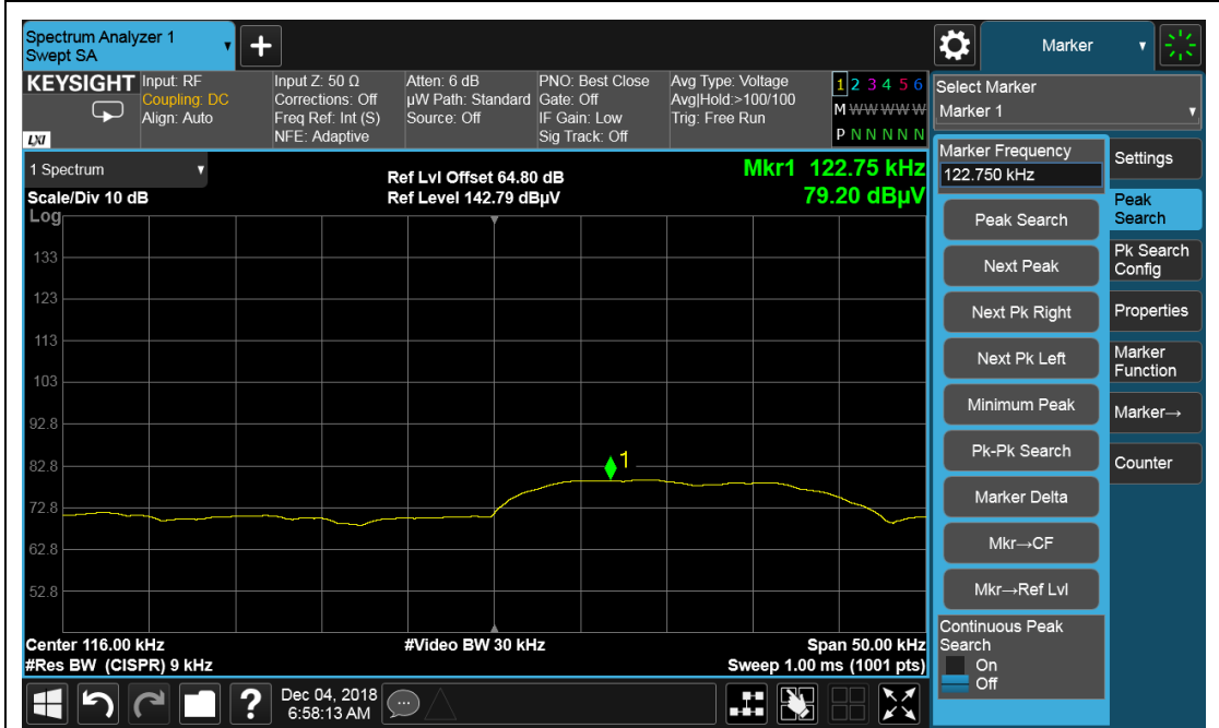
2 nd harmonic – 116kHz
