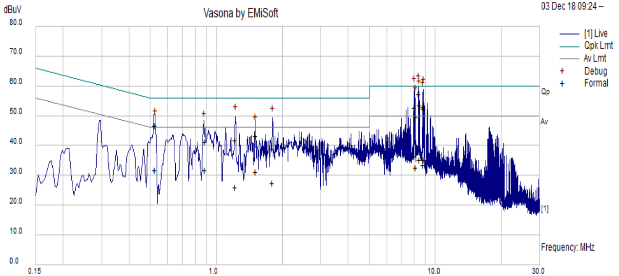
Power Line Conducted Emissions Template: AC Cond Emi Class B Line Filename: c:\program files\emisoft - vasonaresults\SEN-005 120V 60H Line.emi
