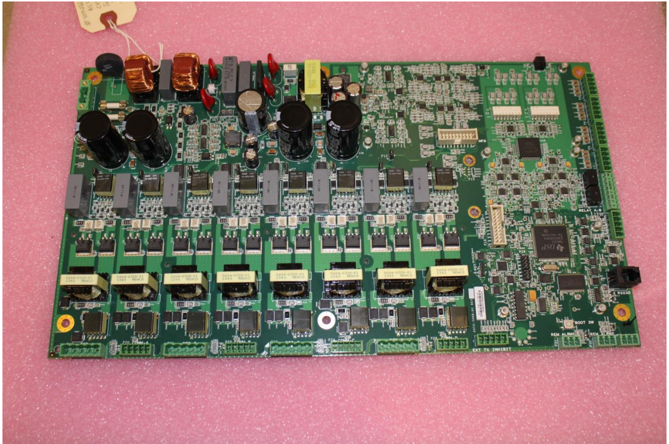
EUT Photos. 4 channel version
