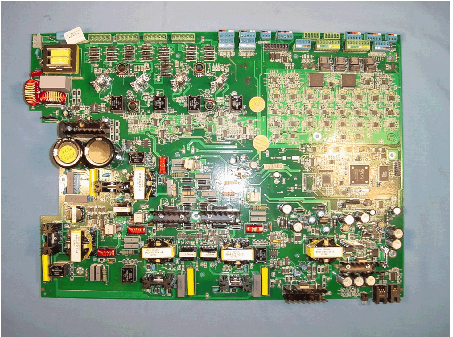
Internal Photo 2 – Board Top View
