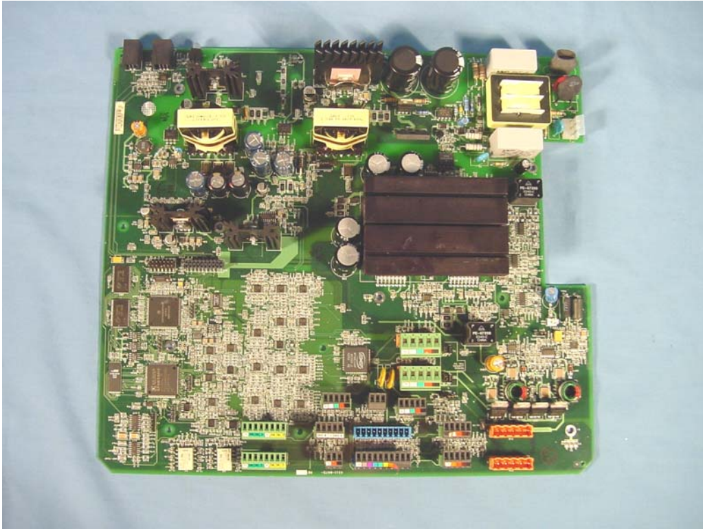
Internal Photo 2 – Board Top View
