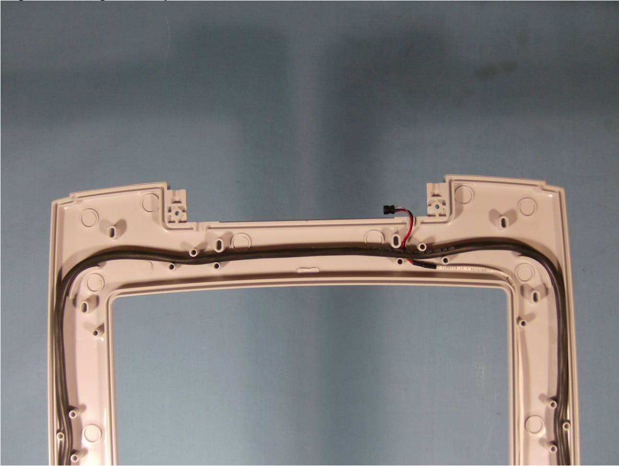
Top end of Loop assembly with Alarm LED cable
