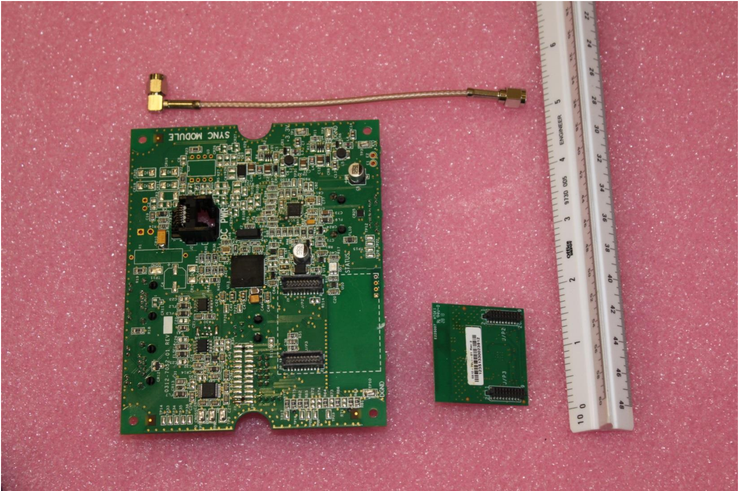
RF board backside with larger digital board and test cable.
