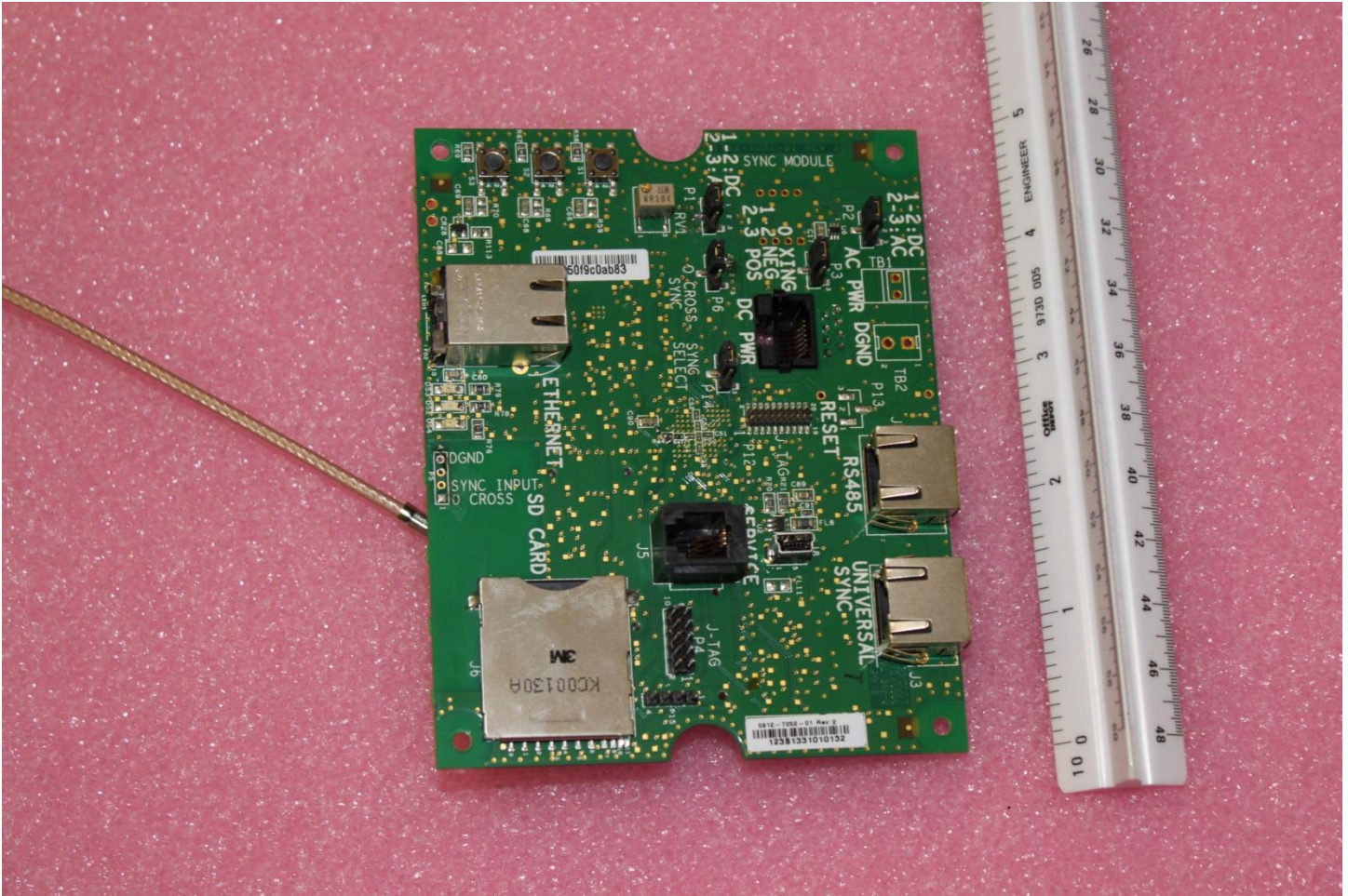
Digital board backside
