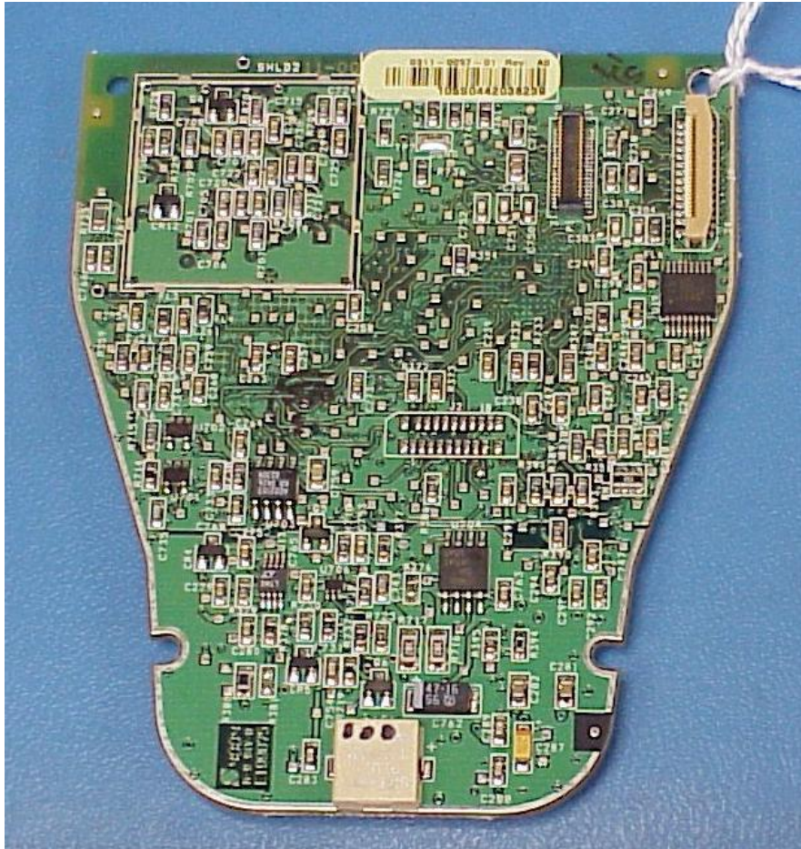
Internal Photo 7 – Pistol Processor PCB Bottom View
