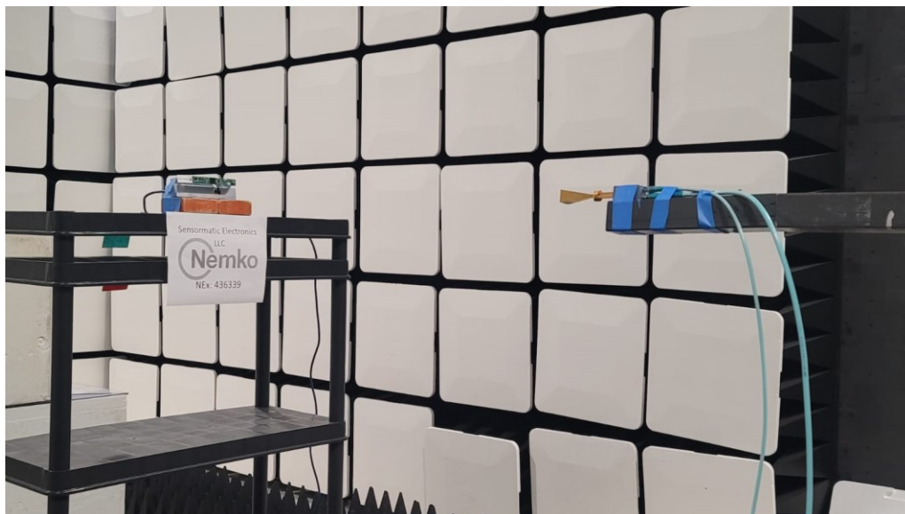
Figure 11 - Radiated emissions above 1 GHz (75 – 110 GHz), front view, 1 meter distance.
