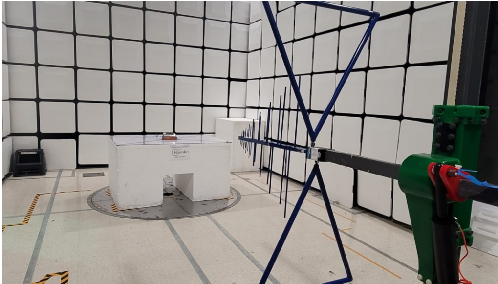
Figure 1 - Radiated emissions below 1 GHz (0.03 – 1 GHz), front view, 3 meters distance.
