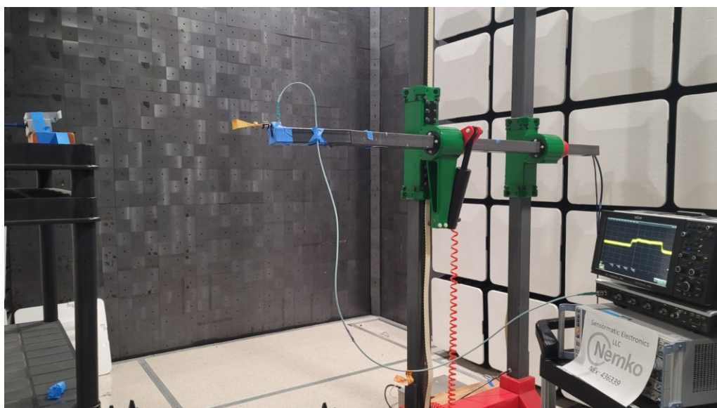
Figure 15 – Test setup (power meter measurements, 0.47 meters distance).
