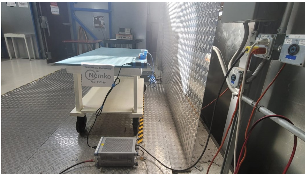
Figure 20 – Conducted emissions test setup.
