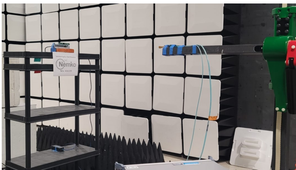
Figure 12 - Radiated emissions above 1 GHz (110 – 140 GHz), front view, 1 meter distance.
