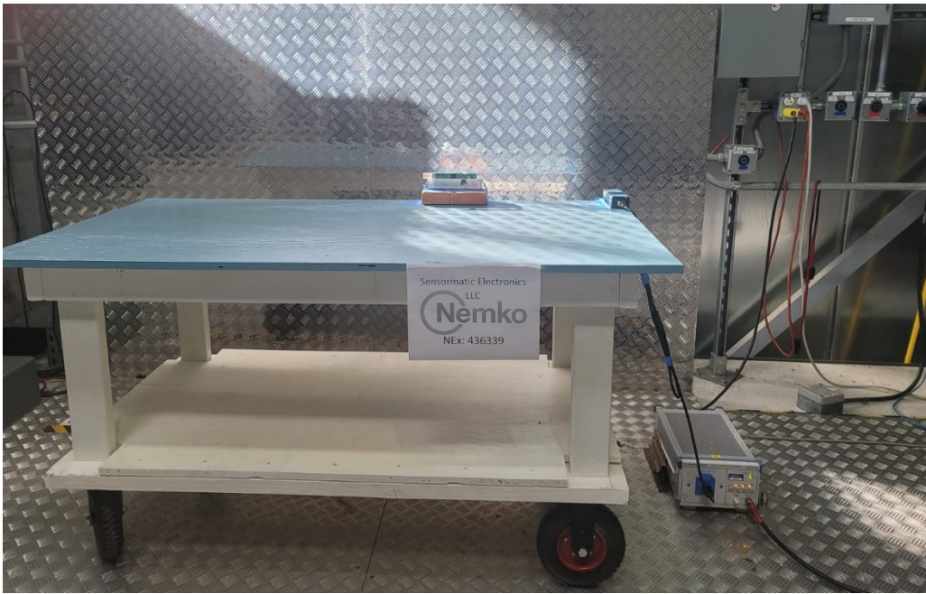
Figure 19 – Conducted emissions test setup.
