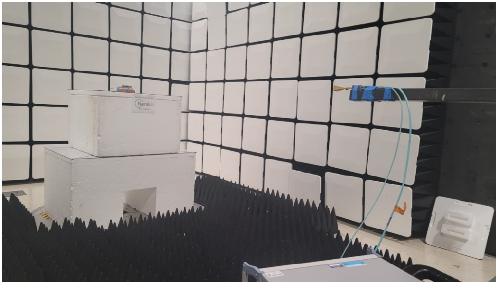
Figure 10 - Radiated emissions and occupied bandwidth tests, above 1 GHz (50 – 75 GHz), front view, 3 meters distance.
