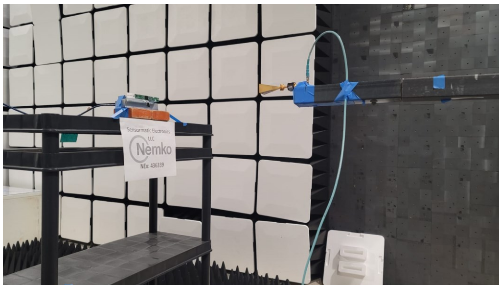
Figure 14 – Test setup (power meter measurements, 0.47 meters distance).
