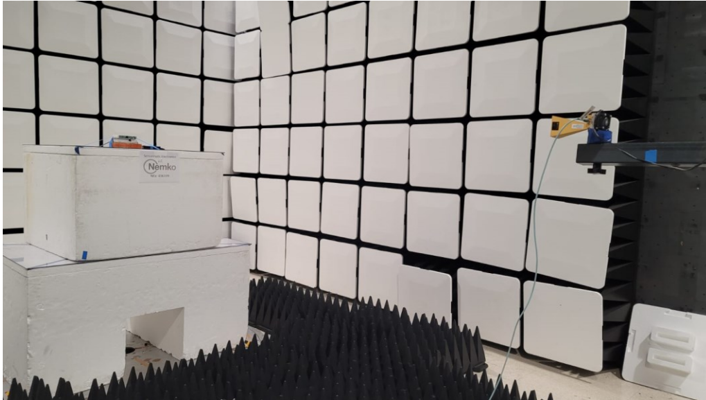
Figure 7 - Radiated emissions above 1 GHz (26 – 40 GHz), front view, 3 meters distance.
