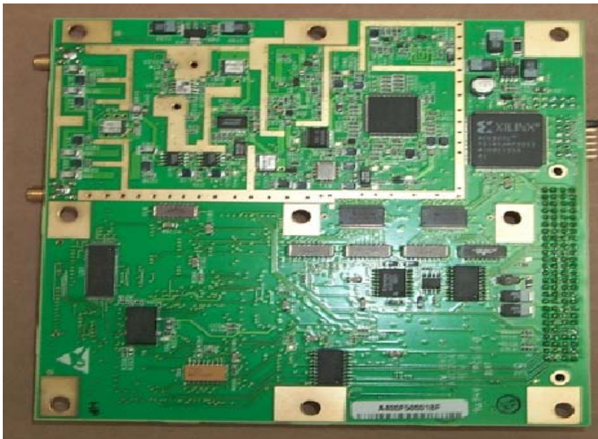
EUT – Layer 2 Main Board Solder View
