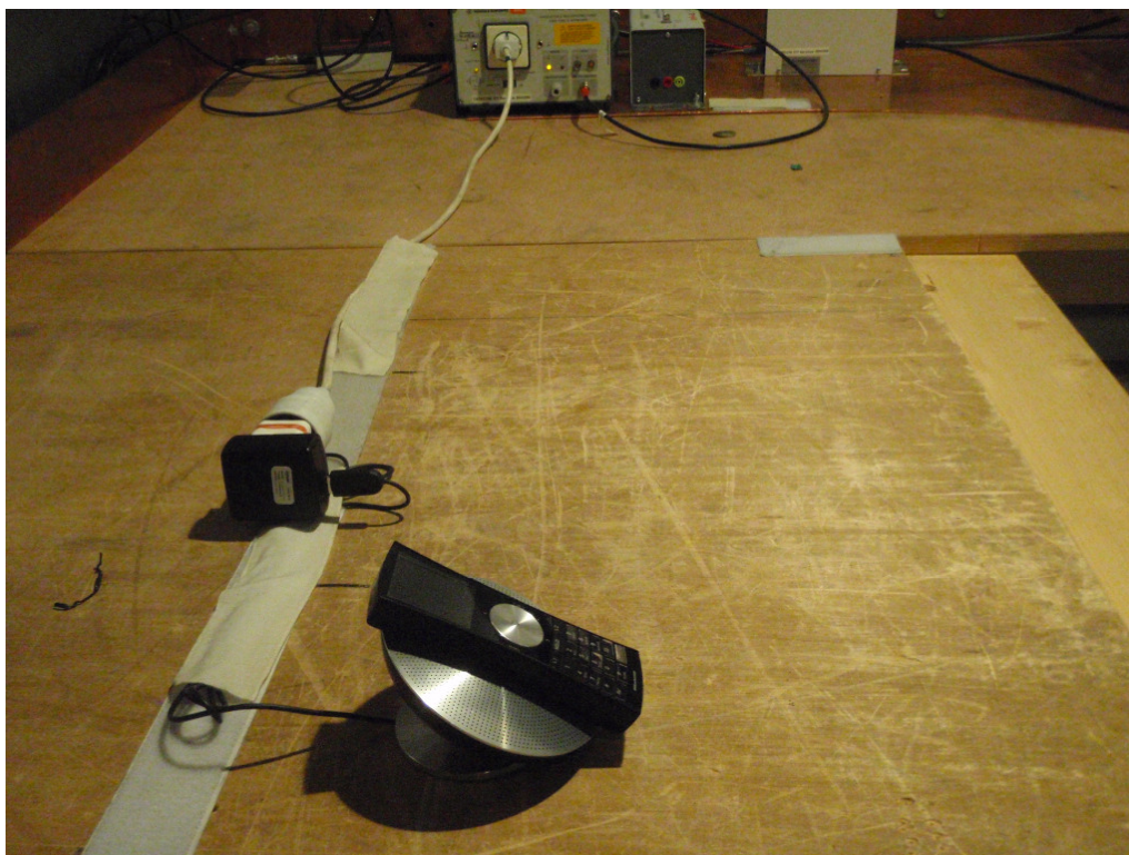
Photo 2: Power Line Conducted Emission Test
