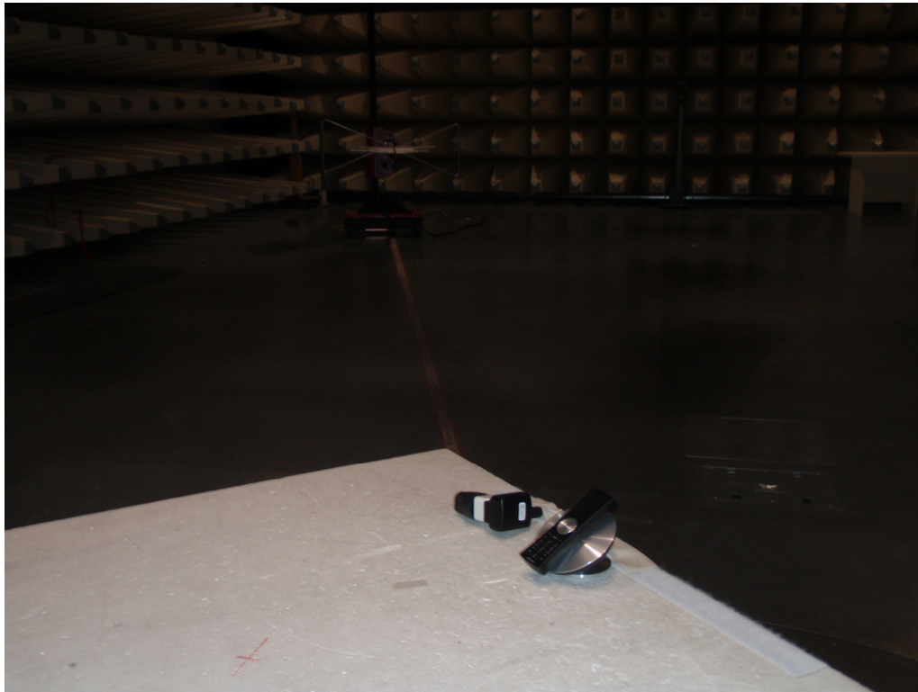
Photo 3: Radiated Emission
