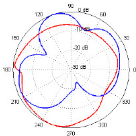
(c) yz-plane, C_\phi (blau, G_{\max} \Rightarrow 1.35 dBi), C_\psi (red, G_{\max} \Rightarrow 14.07 dBi)
