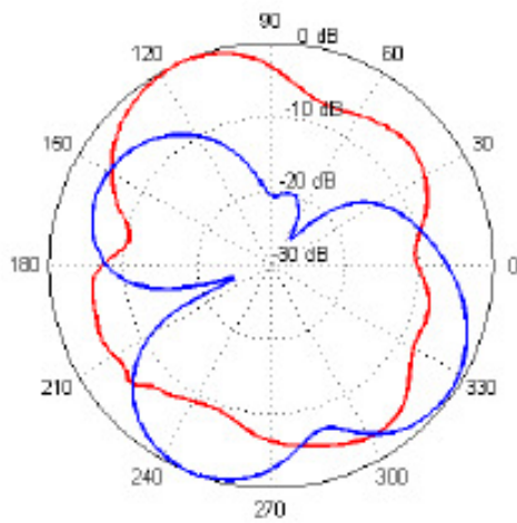
(c) yz-plane, C_\theta (blau, G_{\max} = 2.26 dBi), C_\phi (red, G_{\max} = -12.63 dBi)
