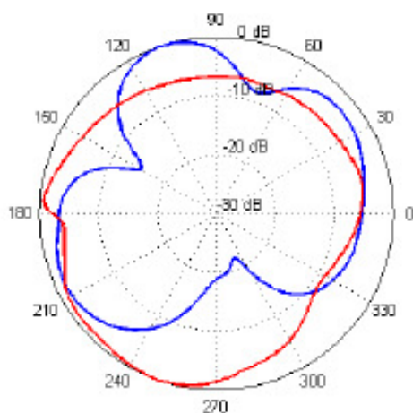
(c) yz-plane, C_\phi (blau, G_{\max} \Rightarrow 1.67 dBi), C_\psi (red, G_{\max} \Rightarrow 14.51 dBi)
