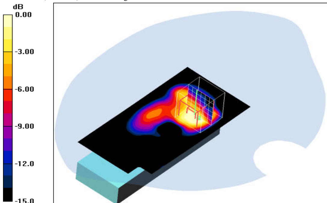
0 dB = 0.017mW/g
