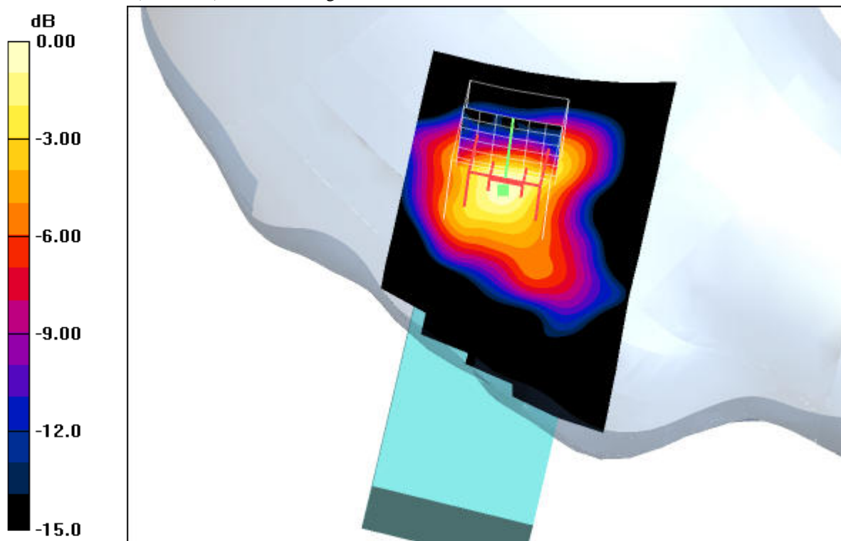
0 dB = 0.013mW/g
