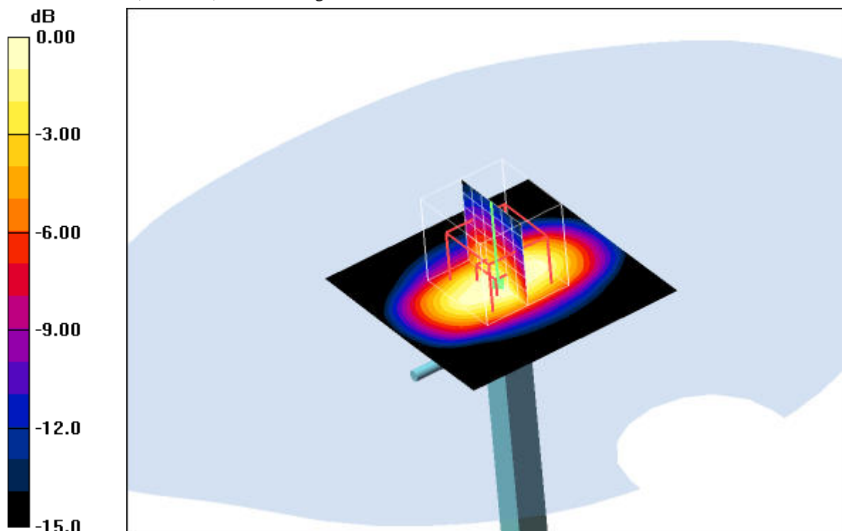
0 dB = 44.5mW/g
