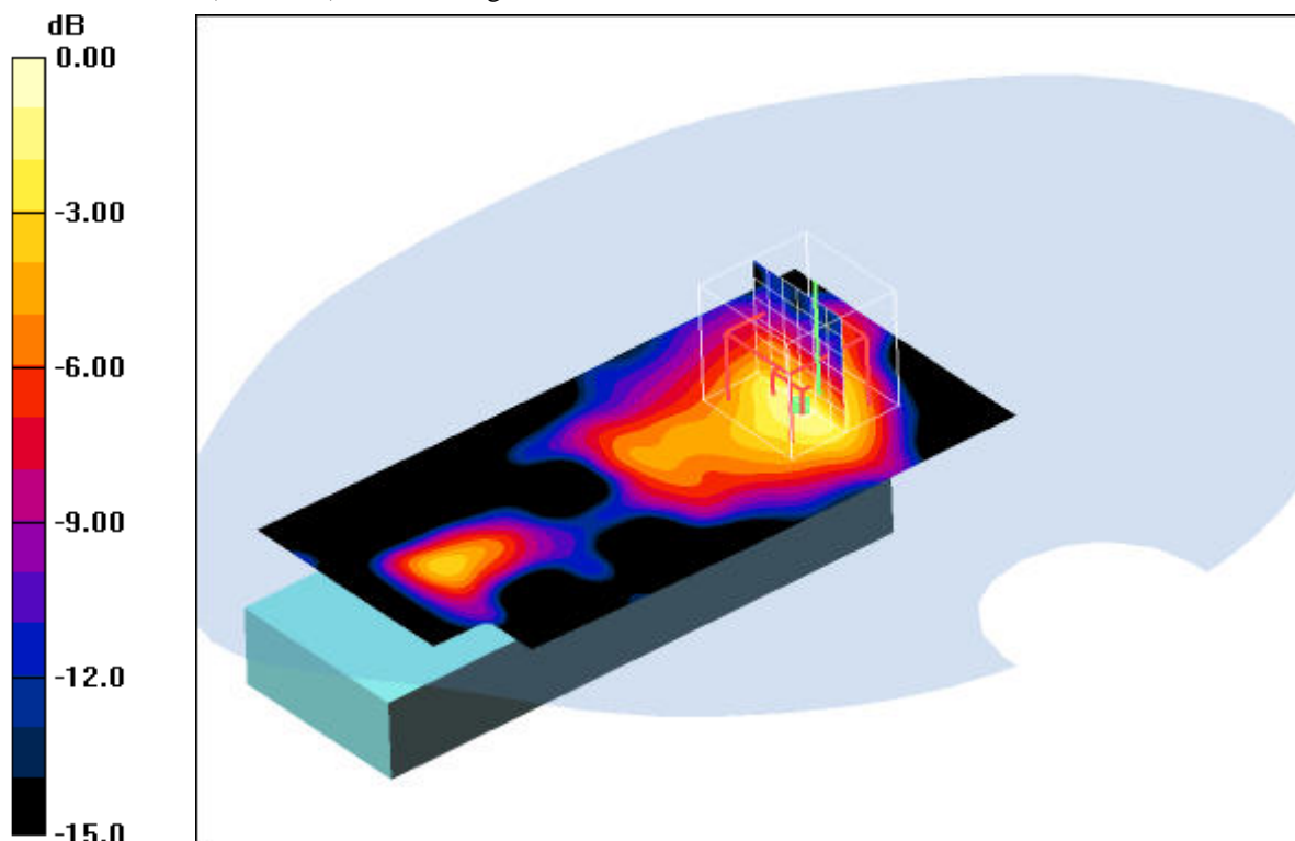
0 dB = 0.010mW/g
