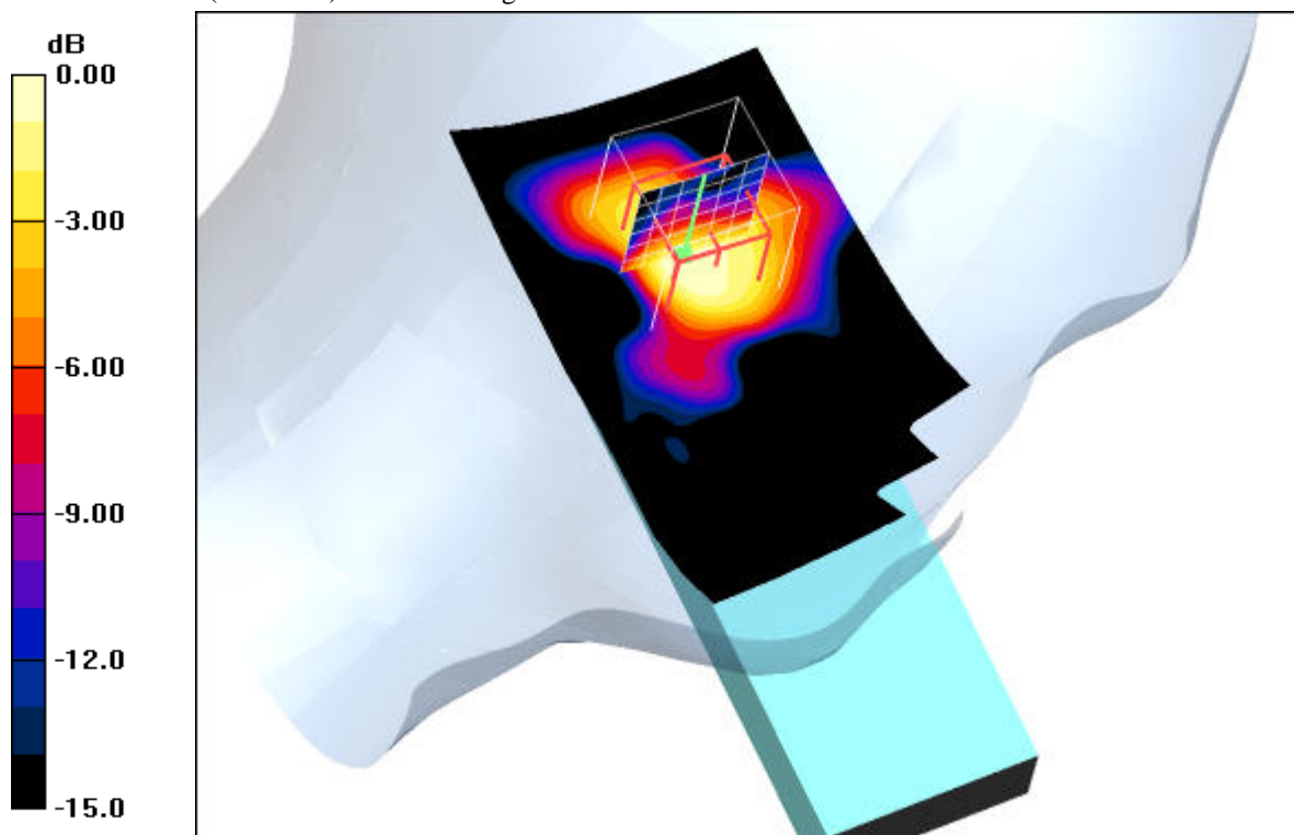
0 dB = 0.011mW/g
