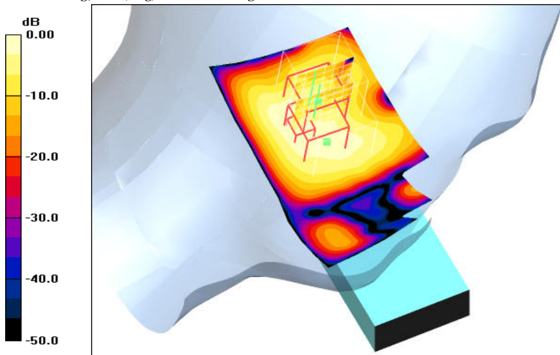
0 dB = 0.010mW/g
