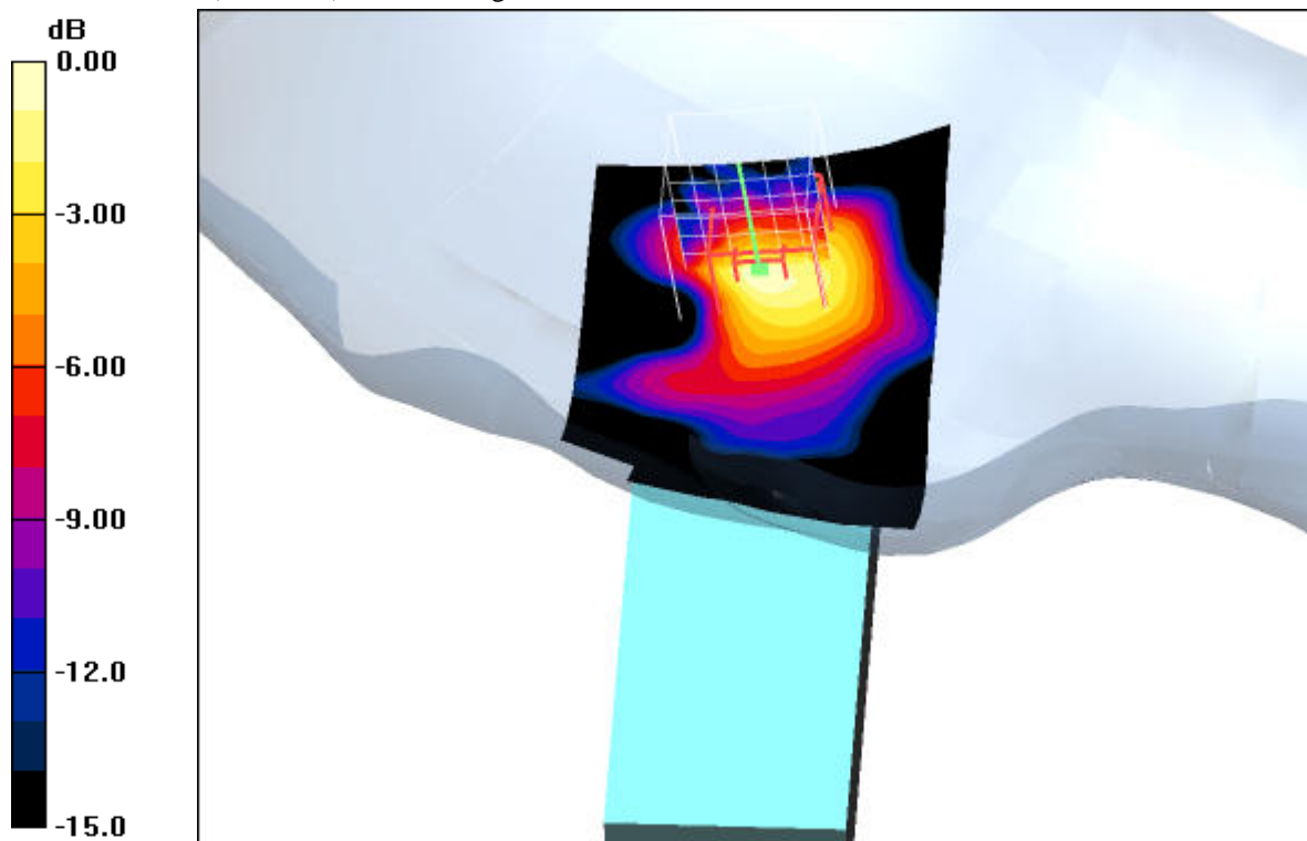
0 dB = 0.010mW/g
