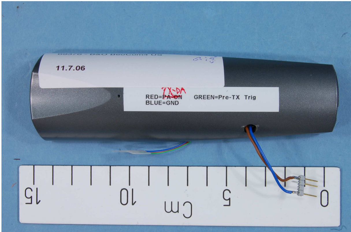
BEOCOM 4 HANDSET
